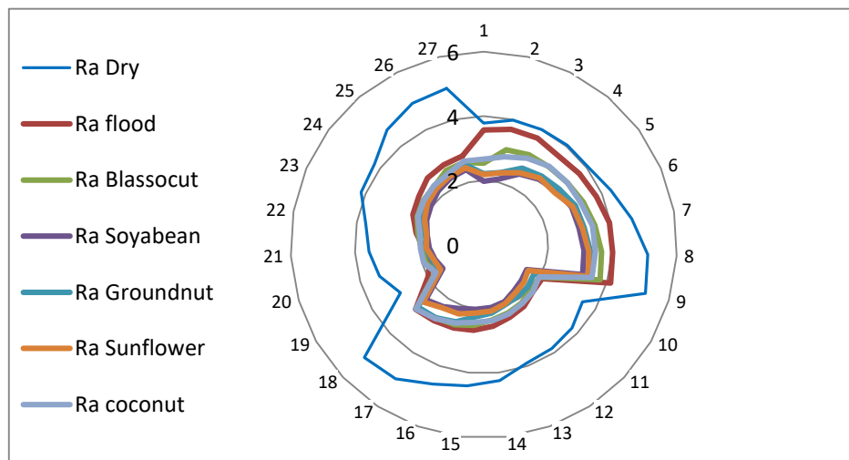
Figure 2. Surface roughness variation of at different cutting condition.
