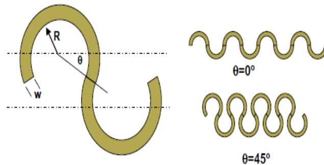
Figure 5. Definition of horseshoe design by its inner radius (R), joining angle ( \theta ) and width of metal track (w) (Gonzalez et al., 2008)
