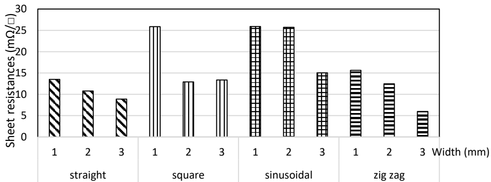
Figure 2. Sheet resistance of different shapes with different widths at the unloaded condition
