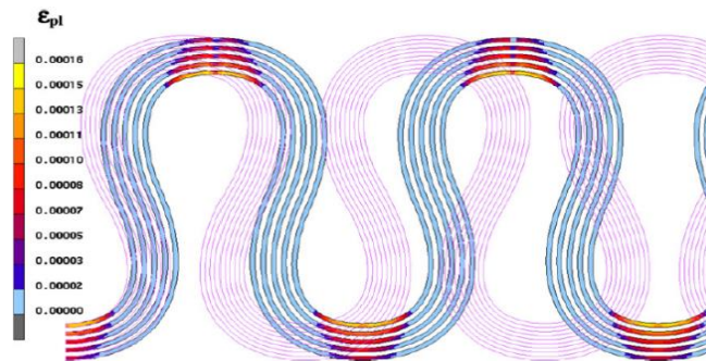
Figure 6. Plastic strain distribution in a multi-track horseshoe conductor design (Gonzalez et al., 2008)
