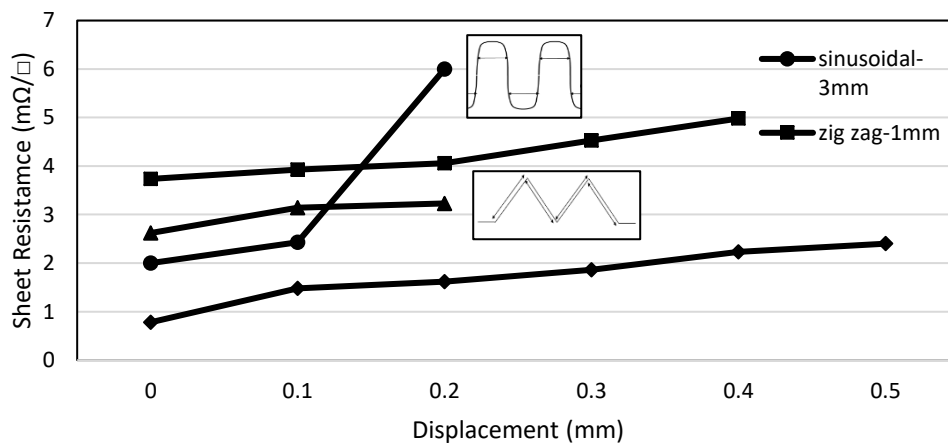
Figure 4. Sheet resistance of different shape at point parallel to the applied stretch
