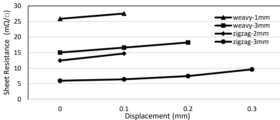
Figure 3. Sheet resistance of different shape when elongate at different displacement
