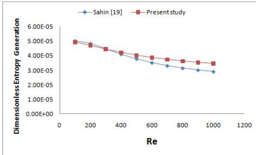
Figure 2. Comparing the present results with the results of Sahin 2008 ( n=1, \theta=0.01 and \phi=0 )
