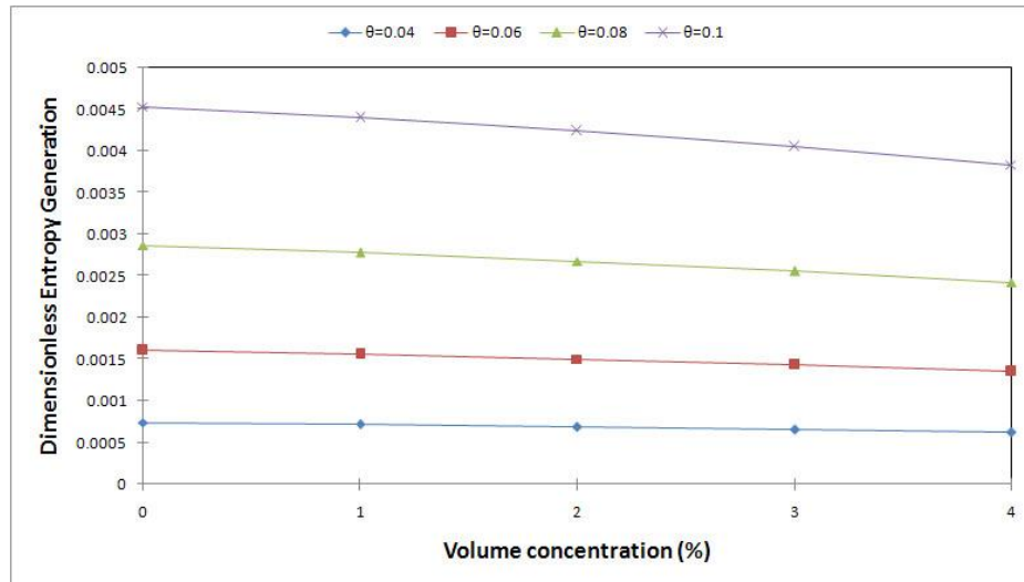
Figure 4. The effect of dimensionless temperature and volume concentration of Al 2 O 3 on dimensionless entropy generation ( n=0.85 , Re=500 )
