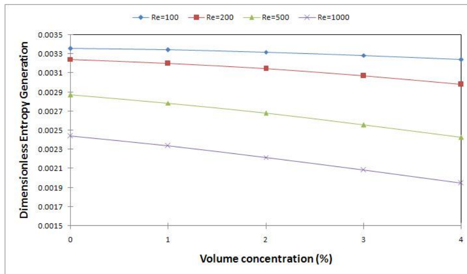
Figure 5. The effect of Reynolds number and volume concentration of Al 2 O 3 on dimensionless entropy generation ( n=0.85 , \theta=0.08 )
