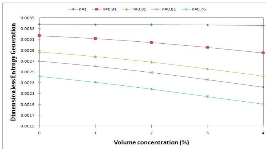
Figure 3. The effect of n and volume concentration of Al_2O_3 on dimensionless entropy generation ( \theta=0.08, Re=500 )
