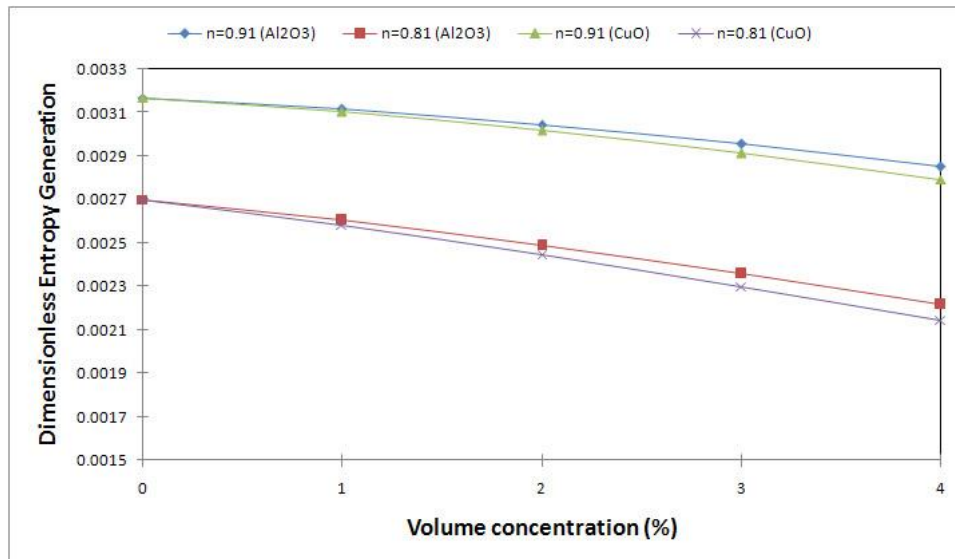
Figure 6. The effect of Power law number and volume concentration of \text{Al}_2\text{O}_3 and \text{CuO} on dimensionless entropy generation ( \text{Re}=500 , \theta=0.08 )
