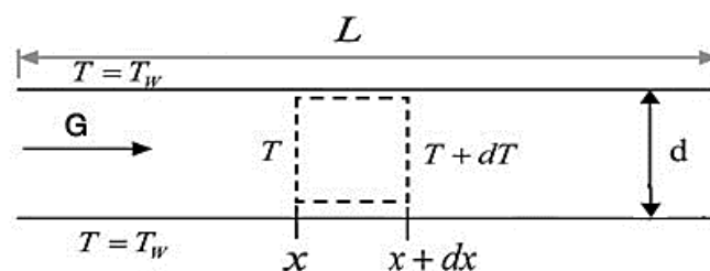
Figure 1. Geometrical configuration
