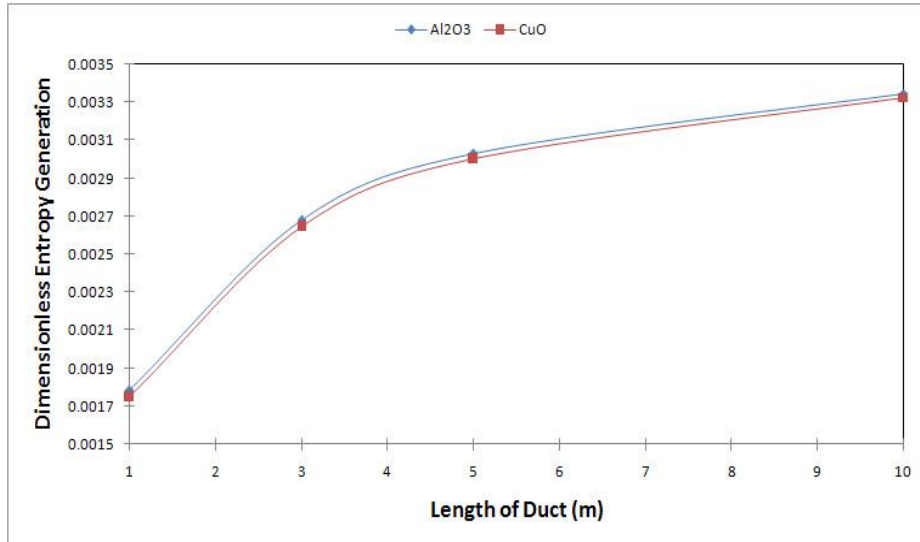
Figure 7. The effect of length of duct and nanoparticles types on dimensionless entropy generation ( n=0.85 , \theta=0.08 , \phi=2\% and Re=500 )
