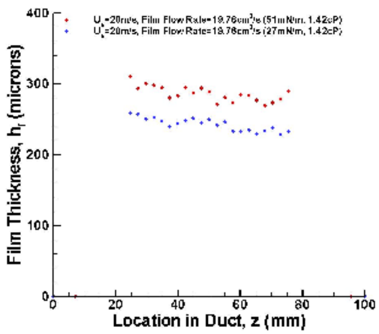
Figure 4.21. Measured film thickness of fluids with different surface tension.
