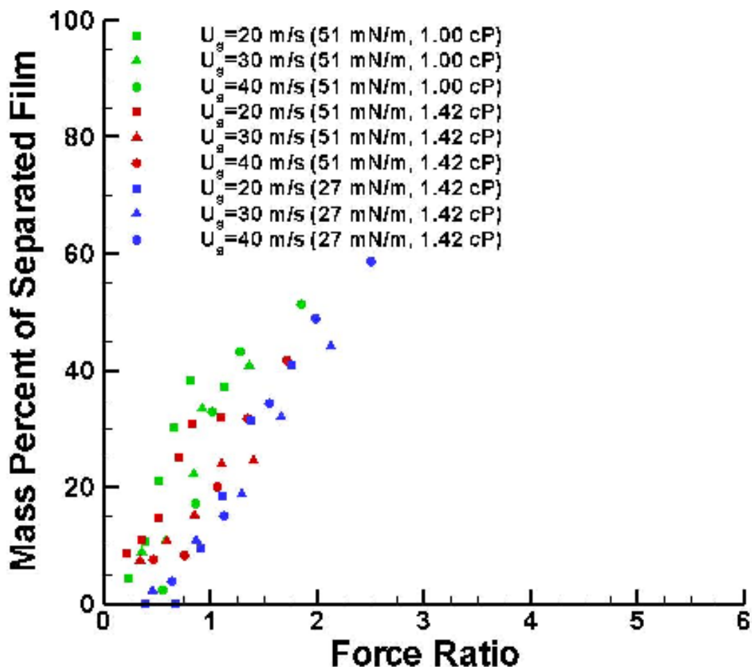
Figure 4.44. Experimentally measured mass percent of film separation plotted versus the Force Ratio of Friedrich et al. [35] for 43 flow conditions. The Force Ratio was calculated using values of film thickness and velocity predicted by the Volume of Fluids model.
