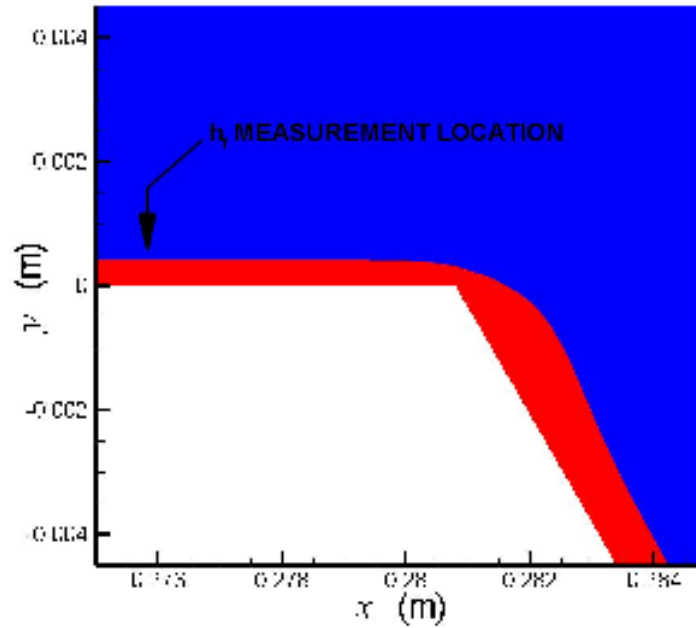
Figure 4.29. The computational results of the Volume of Fluids model for U_g = 20 m/s and \frac{\dot{V}_f}{w_f} = 1.71 cm 2 /s, with surface curvature upstream from the corner.
