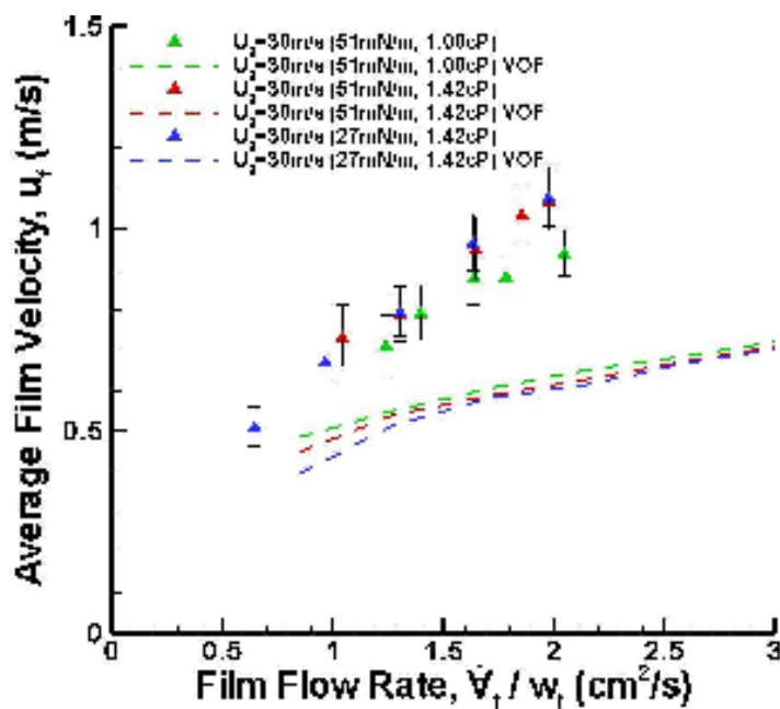
Figure 4.35. Average film velocity as simulated by the Volume of Fluids model plotted with the experimentally determined values of all three fluids for U_g = 30 m/s.
