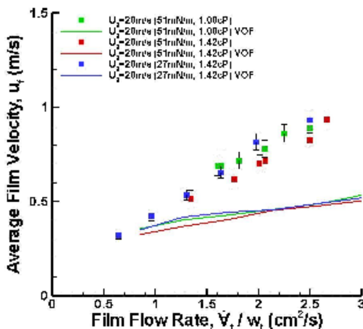
Figure 4.34. Average film velocity as simulated by the Volume of Fluids model plotted with the experimentally determined values of all three fluids for U_g = 20 m/s.
