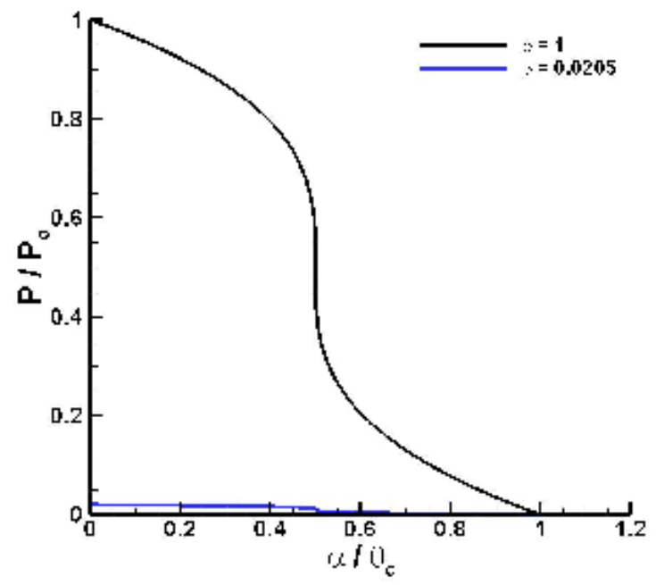
Figure 3.12. The relative power with and without including the reflection coefficient plotted versus the subject surface angle divided by laser cone angle. (top surface reflection)
