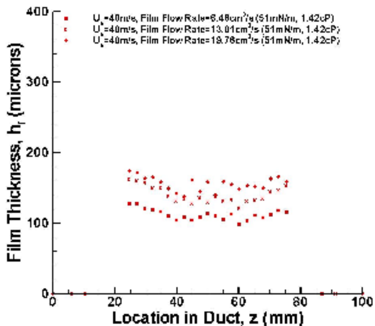
Figure 4.18. Measured film thickness of the glycerol-vinegar mixture for various film flow rates at U_g = 40 m/s.
