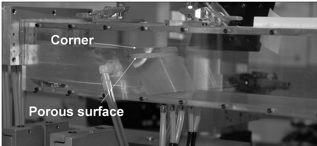
Figure 4.39. Picture of the test section showing the porous surface where the film that remains attached after the corner is removed.
