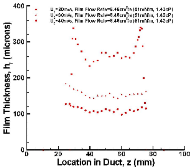
Figure 4.11. Measured film thickness of the glycerol-vinegar mixture for various gas phase velocities at \dot{V}_f = 6.46 \text{ cm}^3/\text{s} .
