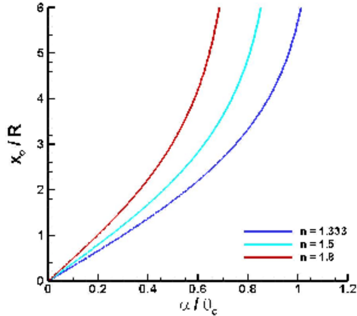
Figure 3.8. The reflected laser center location plotted versus the subject surface angle, normalized by the incident cone radius and the cone angle, respectively. (bottom surface reflection)
