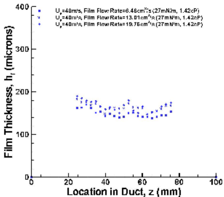
Figure 4.20. Measured film thickness of oil for various film flow rates at U_g = 40 m/s.
