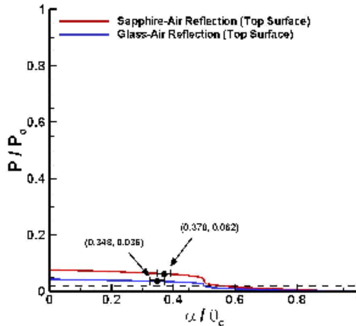
Figure 3.23. Relative power plotted versus surface angle divided by laser cone angle. The estimated minimum relative power is shown, including points representing the maximum measurable angle for each material.
