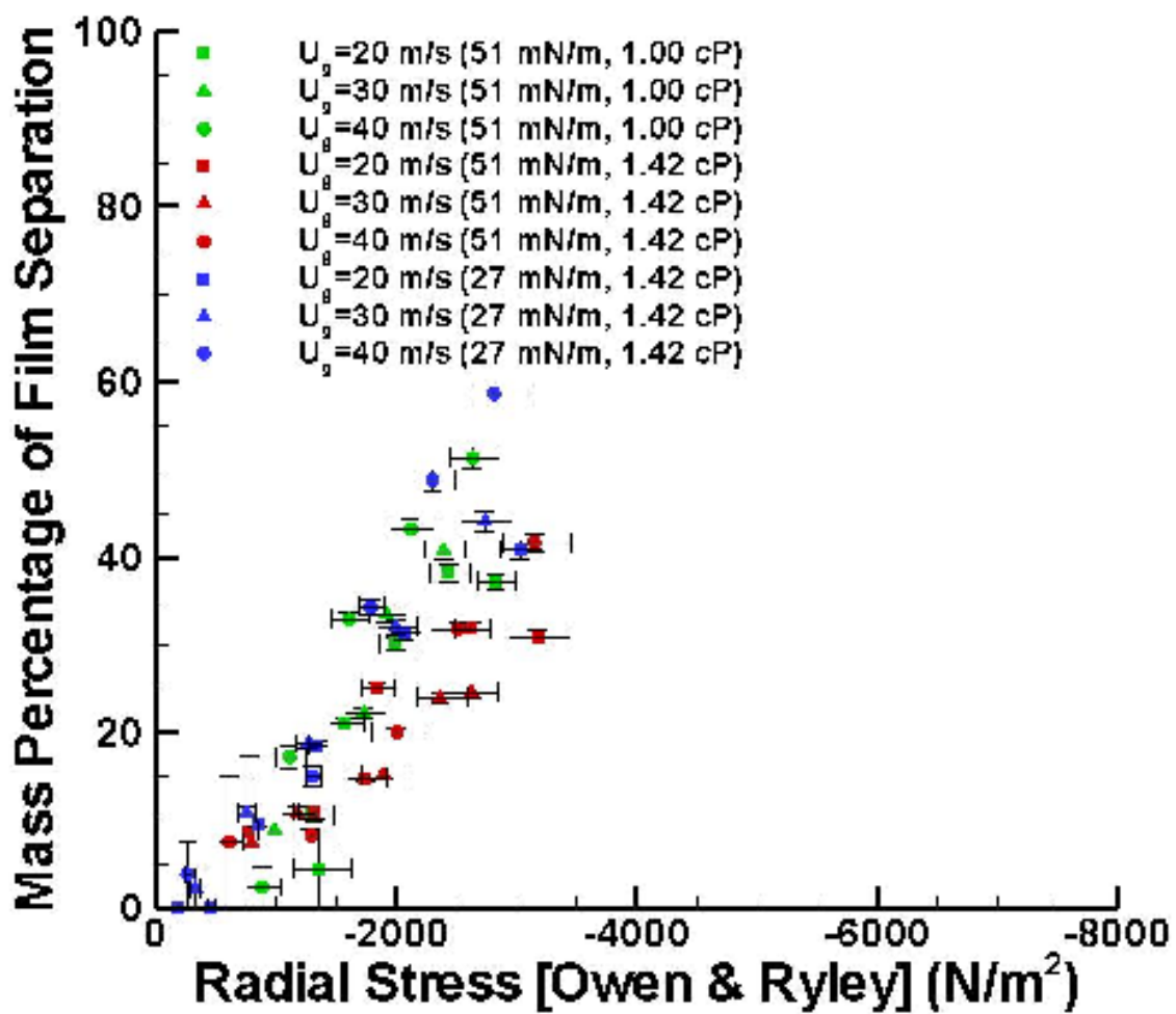
Figure 4.48. Experimentally measured mass percent of film separation plotted versus radial stress of Owen and Ryley [27] for 43 flow conditions. Radial stress was calculated using experimentally measured values of film thickness and velocity.
