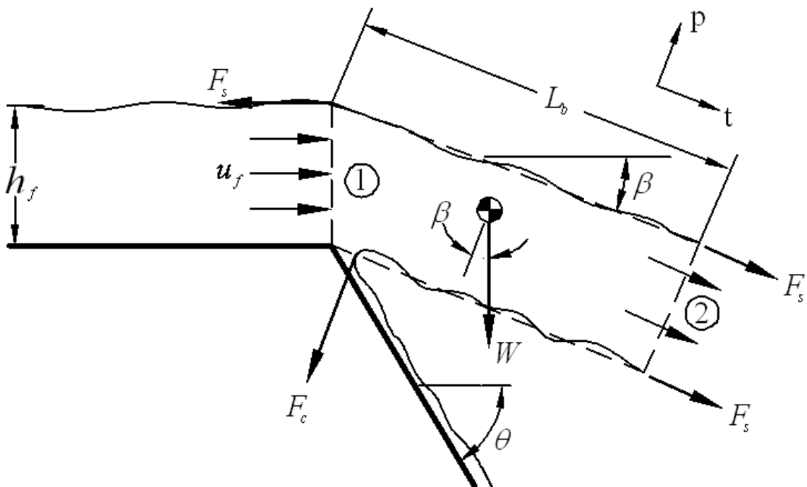
Figure 4.42. Force diagram of a film ligament at the point of separation. (Friedrich et al. [35])
