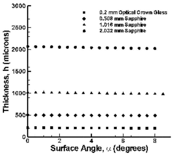
Figure 3.20. Thickness measurements for four different subjects when at various angles of orientation.
