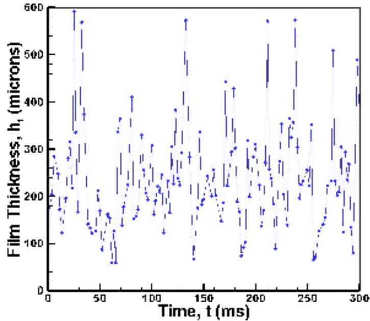
Figure 4.2. Time resolved film thickness measured using a laser focus displacement instrument.
