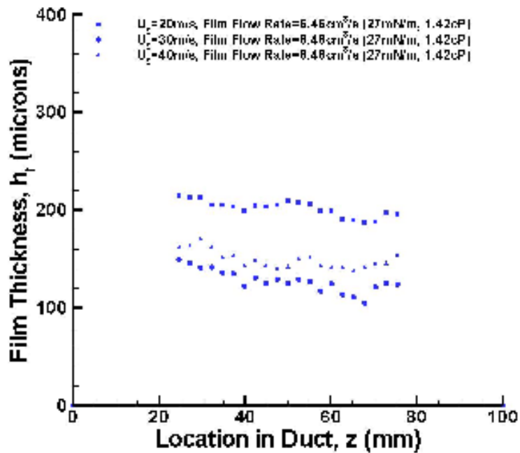
Figure 4.13. Measured film thickness of oil for various gas phase velocities at \dot{V}_f = 6.46 \text{ cm}^3/\text{s} .
