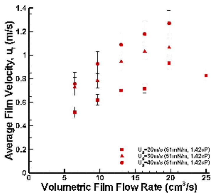
Figure 4.24. Average film velocity of the glycerol-vinegar mixture for various gas phase velocities.
