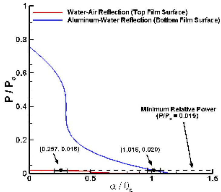
Figure 3.19. Relative power plotted versus surface angle divided by laser cone angle. The estimated minimum relative power is shown, including points of intersection.
