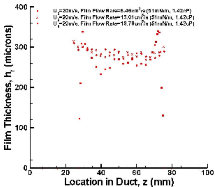
Figure 4.17. Measured film thickness of the glycerol-vinegar mixture for various film flow rates at U_g = 20 m/s.
