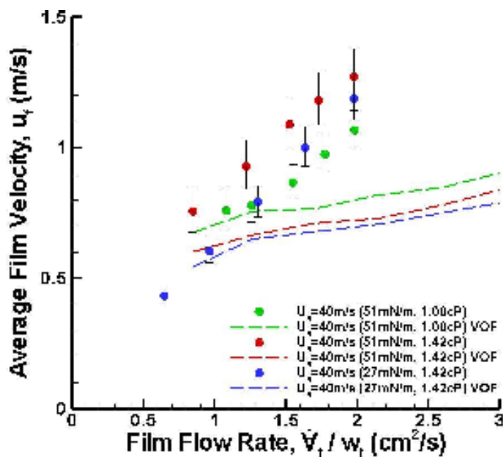
Figure 4.36. Average film velocity as simulated by the Volume of Fluids model plotted with the experimentally determined values of all three fluids for U_g = 40 m/s.
