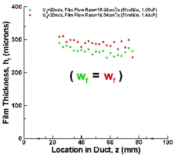
Figure 4.22. Measured film thickness of fluids with different viscosities.
