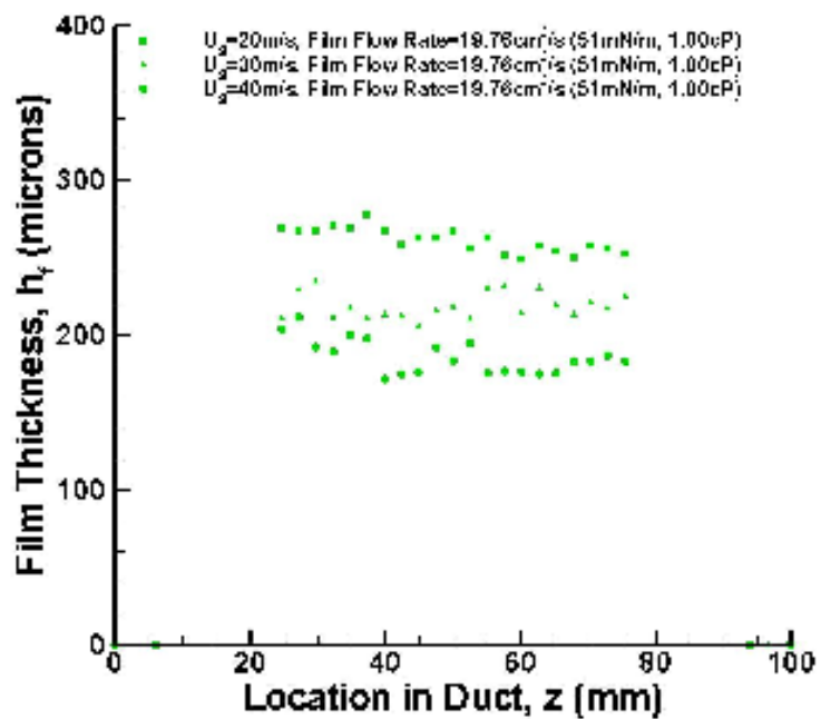
Figure 4.10. Measured film thickness of vinegar for various gas phase velocities at \dot{V}_f = 19.76 \text{ cm}^3/\text{s} .
