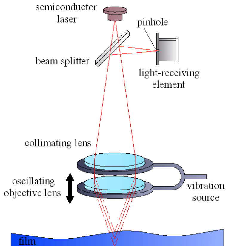
Figure 3.1. Laser focus displacement measuring unit diagram.
