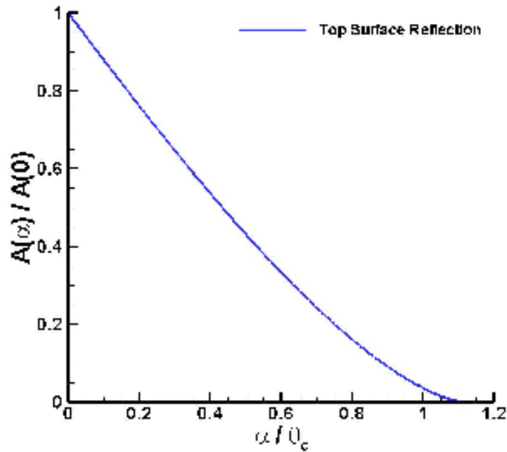
Figure 3.4. Relative area of the reflected light from top surface reflection plotted versus surface angle.
