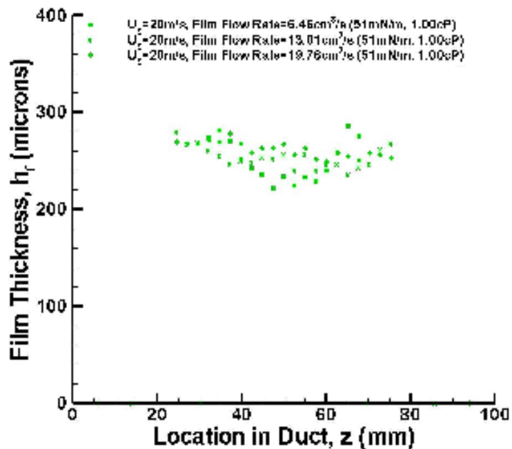
Figure 4.15. Measured film thickness of vinegar for various film flow rates at U_g = 20 m/s.
