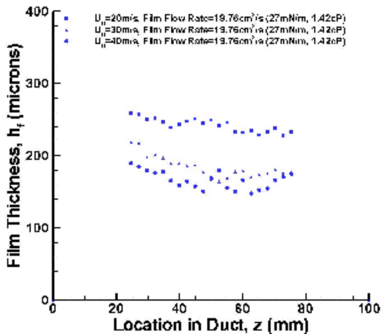
Figure 4.14. Measured film thickness of oil for various gas phase velocities at \dot{V}_f = 19.76 \text{ cm}^3/\text{s} .
