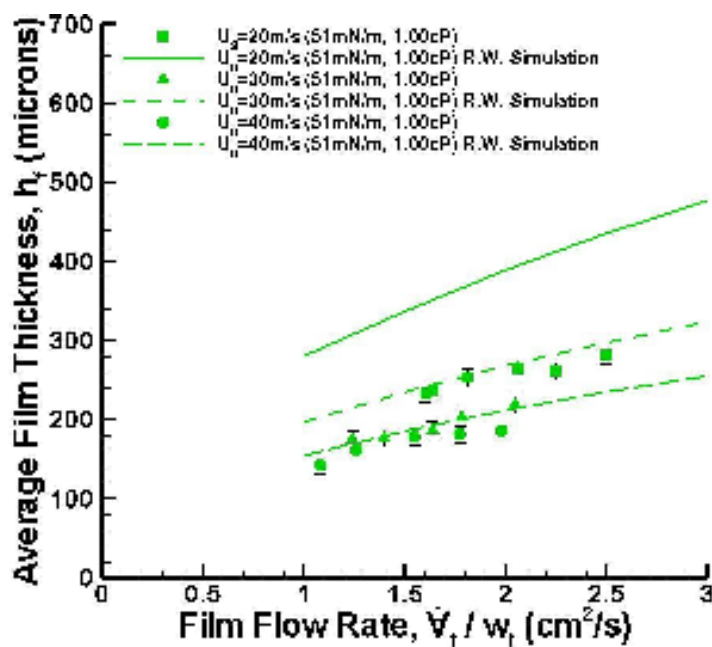
Figure 4.37. Average film thickness as simulated by the Rough Wall Model plotted with the experimentally measured values for vinegar.
