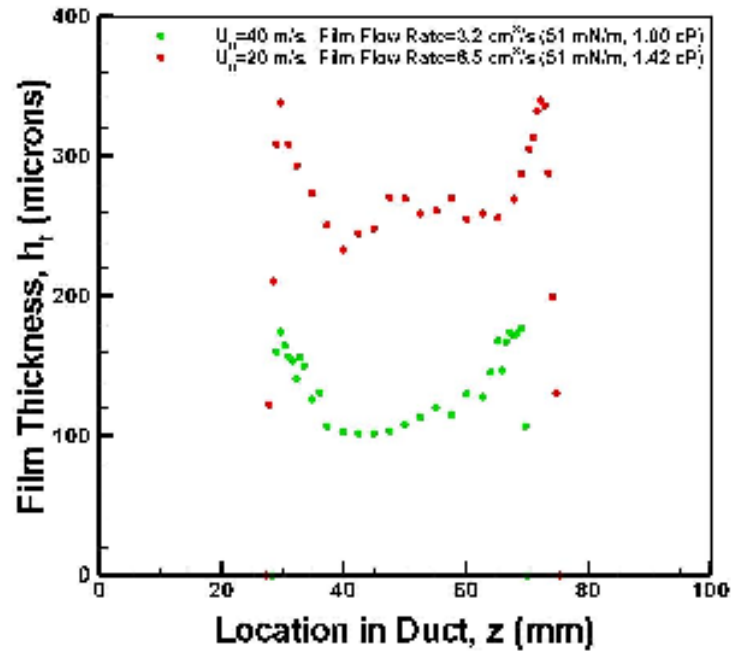
Figure 4.8. An example of film thickness measured across the width of the film.
