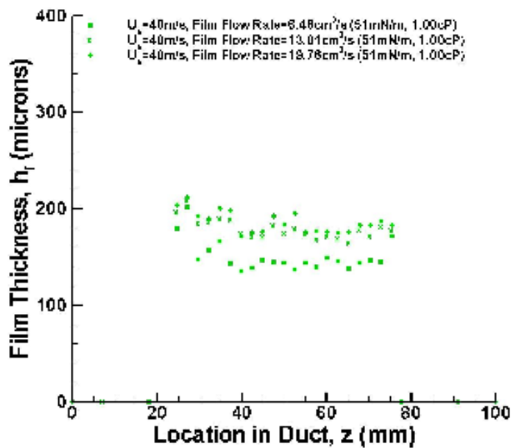
Figure 4.16. Measured film thickness of vinegar for various film flow rates at U_g = 40 m/s.
