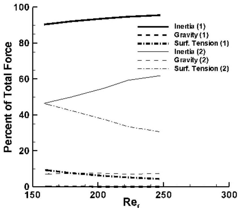
Figure 4.47. Comparison of force balance contribution for the radial stress model of Owen and Ryley [27] (1) and the Force Ratio model of Friedrich et al. [35] (2) at U_g = 20 m/s.
