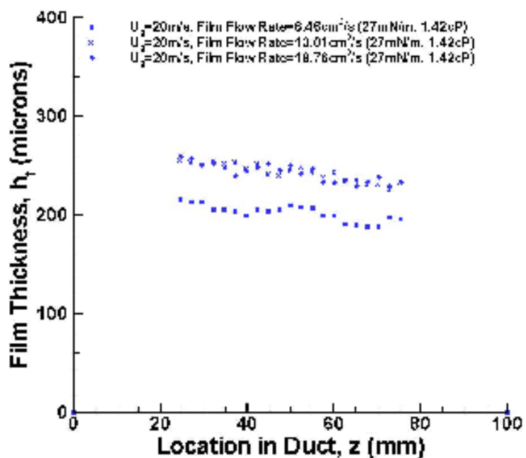
Figure 4.19. Measured film thickness of oil for various film flow rates at U_g = 20 m/s.
