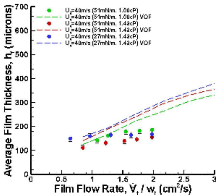
Figure 4.33. Average film thickness as simulated by the Volume of Fluids model plotted with the experimentally measured values of all three fluids for U_g = 40 m/s.
