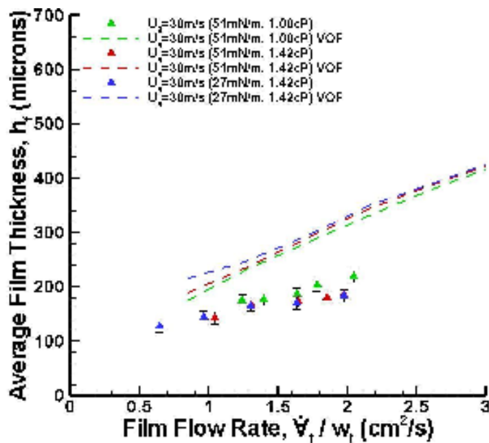
Figure 4.32. Average film thickness as simulated by the Volume of Fluids model plotted with the experimentally measured values of all three fluids for U_g = 30 m/s.
