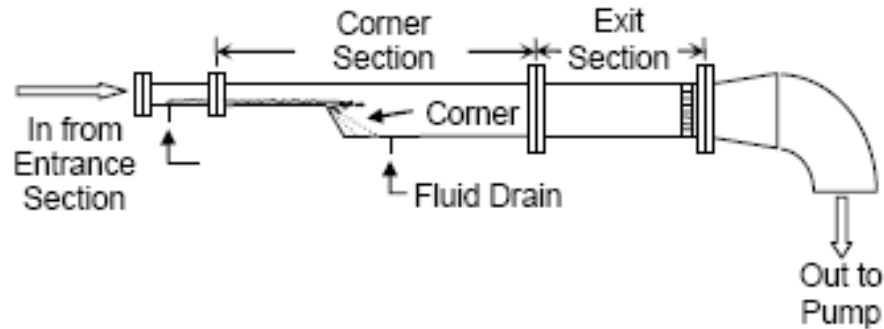
Figure 4.1. Schematic of experimental test section.
