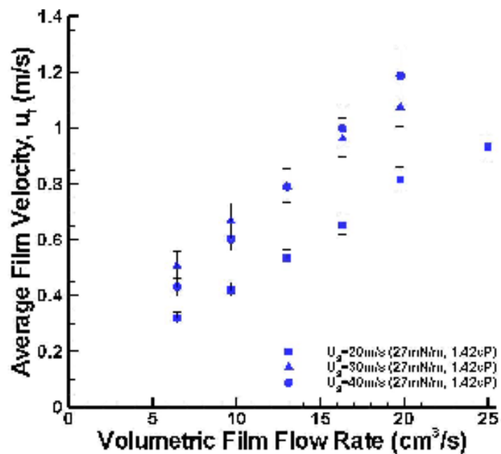
Figure 4.25. Average film velocity of oil for various gas phase velocities.
