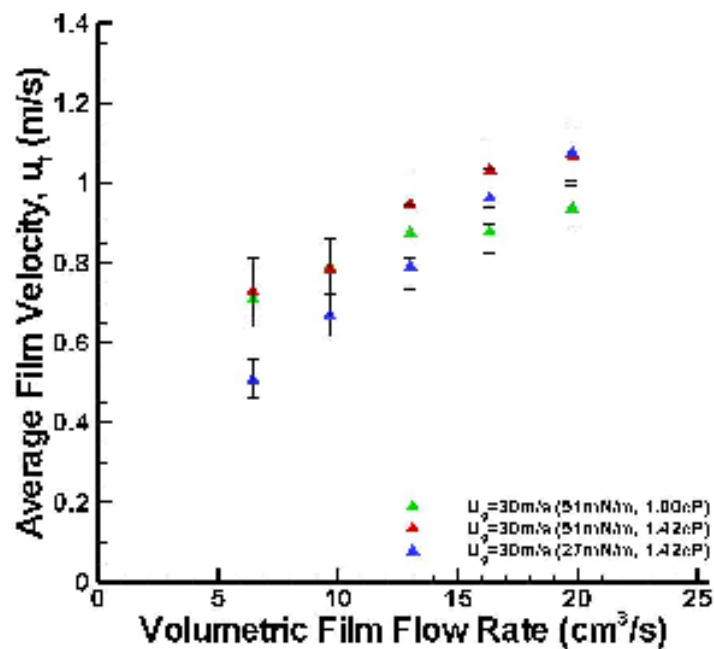
Figure 4.27. Average film velocity of all three fluids for U_g = 30 m/s.
