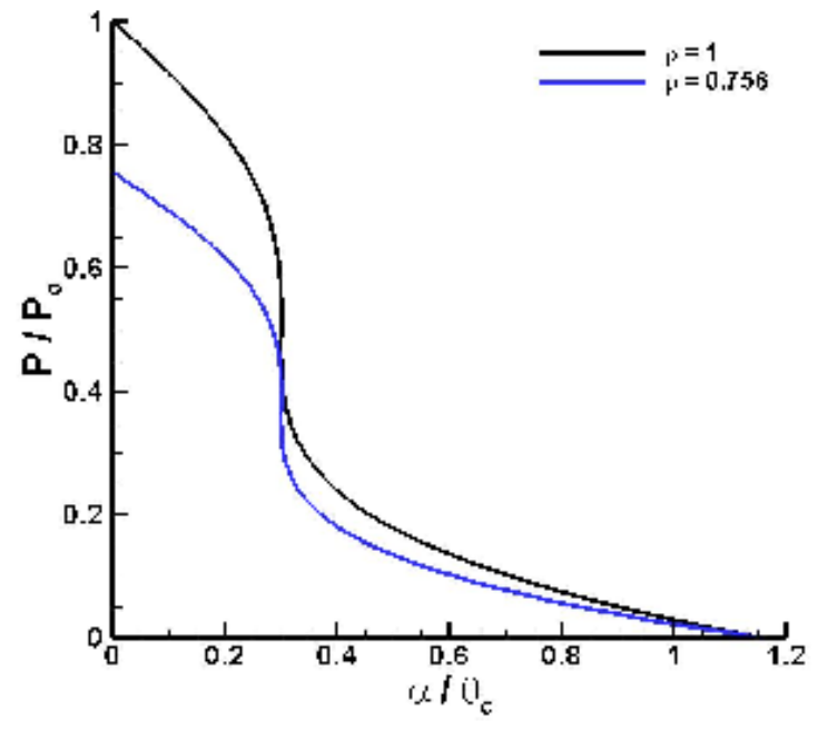
Figure 3.13. The relative power with and without including the reflection coefficient plotted versus the subject surface angle divided by laser cone angle. (bottom surface reflection)
