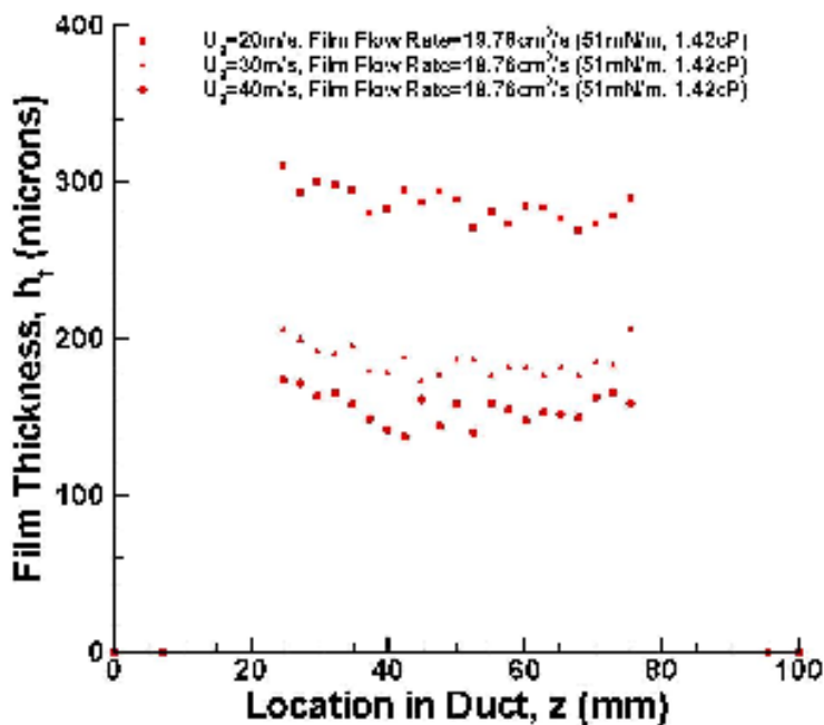
Figure 4.12. Measured film thickness of the glycerol-vinegar mixture for various gas phase velocities at \dot{V}_f = 19.76 \text{ cm}^3/\text{s} .
