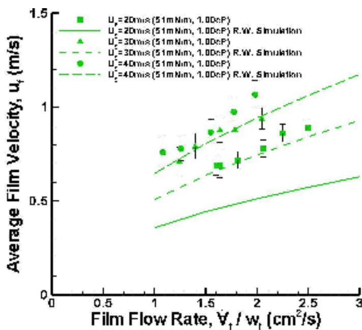
Figure 4.38. Average film velocity as simulated by the Rough Wall Model plotted with the experimentally determined values for vinegar.
