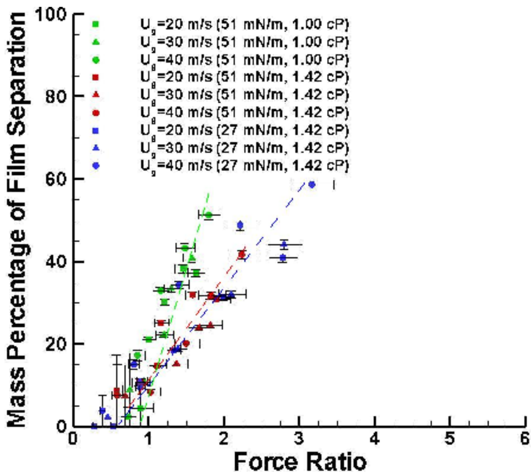
Figure 4.43. Experimentally measured mass percent of film separation plotted versus the Force Ratio of Friedrich et al. [35] for 43 flow conditions. The Force Ratio was calculated using experimentally measured values of film thickness and velocity.
