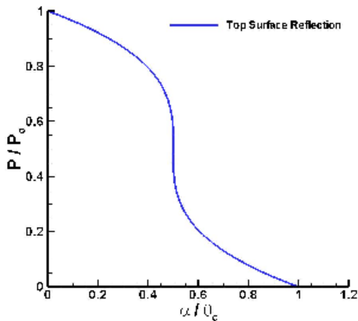
Figure 3.9. The relative power plotted versus the subject surface angle divided by laser cone angle. (top surface reflection)
