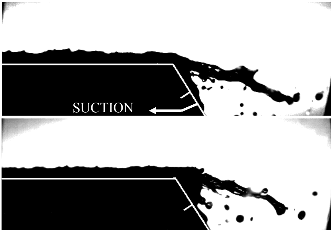
Figure 4.40. High speed images for a surfactant-water mixture at a volumetric film flow rate of 13.01 \text{ cm}^3/\text{s} , and a gas phase velocity of 40 \text{ m/s} . (Top: with negative pressure applied at a drain 6 \text{ mm} downstream from the corner; Bottom: without negative pressure)
