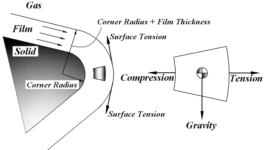
Figure 4.46. Diagram for Radial Stress Model of Owen and Ryley [27].
