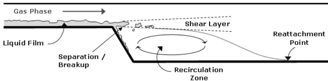
Figure 1.1. Schematic of shear-driven film interaction with separated gas phase flow resulting in partial film separation from the substrate at the corner.
