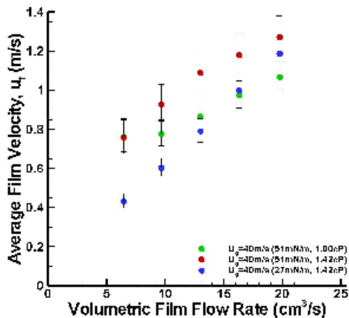
Figure 4.28. Average film velocity of all three fluids for U_g = 40 m/s.
