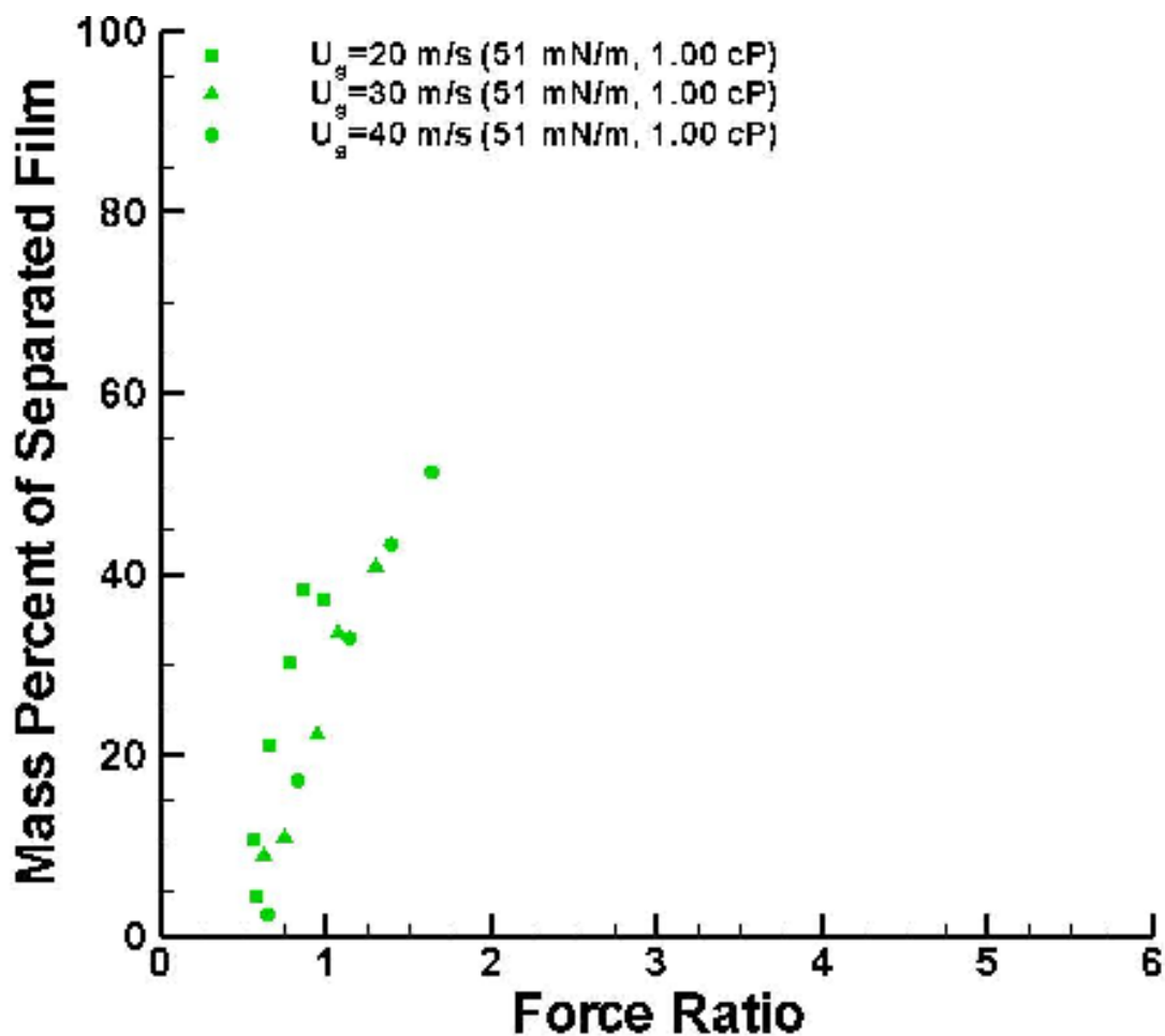
Figure 4.45. Experimentally measured mass percent of film separation plotted versus the Force Ratio of Friedrich et al. [35] for 16 flow conditions. The Force Ratio was calculated using values of film thickness and velocity predicted by the Rough Wall Model.
