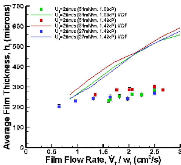
Figure 4.31. Average film thickness as simulated by the Volume of Fluids model plotted with the experimentally measured values of all three fluids for U_g = 20 m/s.
