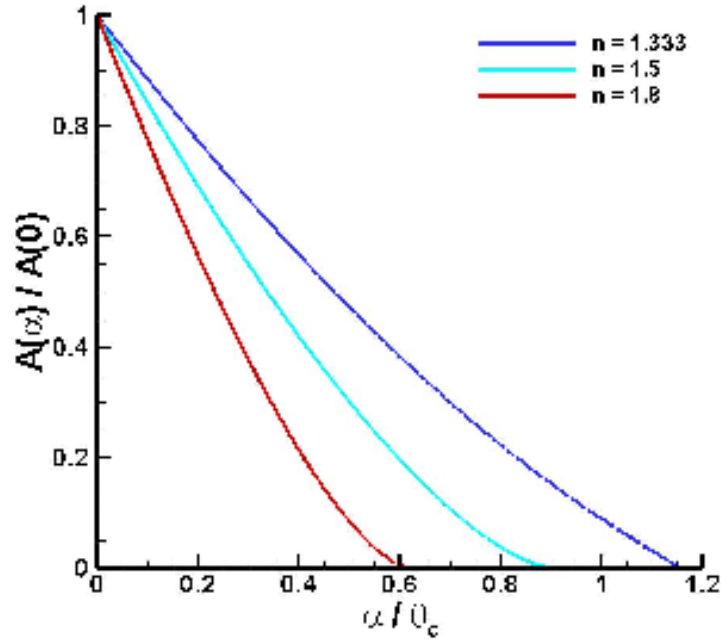
Figure 3.7. The relative area of the reflected light from bottom surface reflection plotted versus surface angle.
