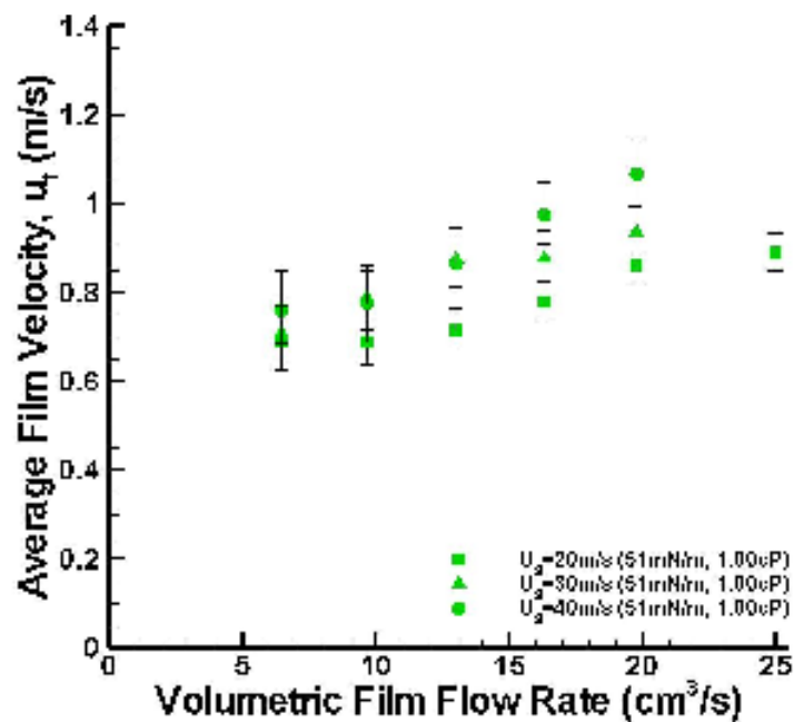
Figure 4.23. Average film velocity of vinegar for various gas phase velocities.
