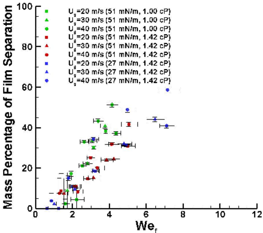
Figure 4.41. Experimentally measured mass percent of film separation plotted versus the film Weber number for 43 flow conditions. The Weber number was calculated using experimentally measured values of film thickness and velocity.
