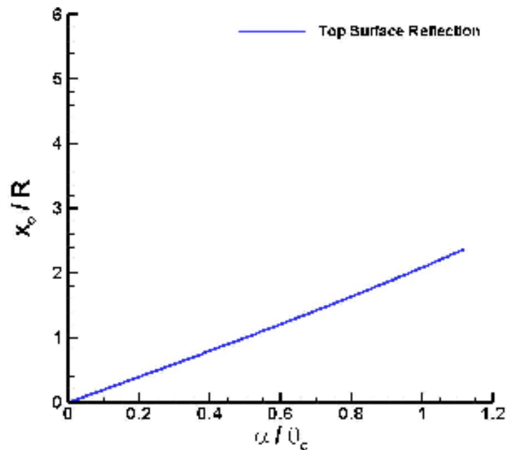
Figure 3.5. The reflected laser center location plotted versus the subject surface angle, normalized by the incident cone radius and the cone angle, respectively. (top surface reflection)
