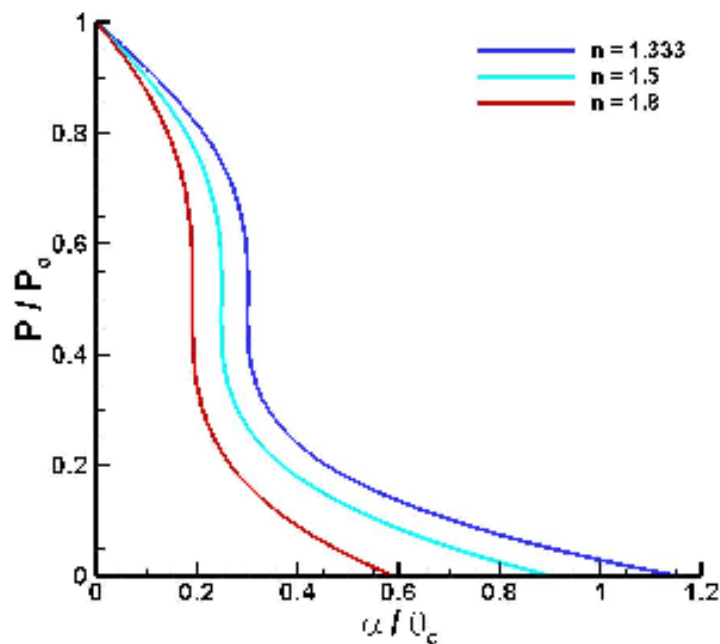
Figure 3.10. The relative power for 3 refractive index values plotted versus the subject surface angle divided by laser cone angle. (bottom surface reflection)
