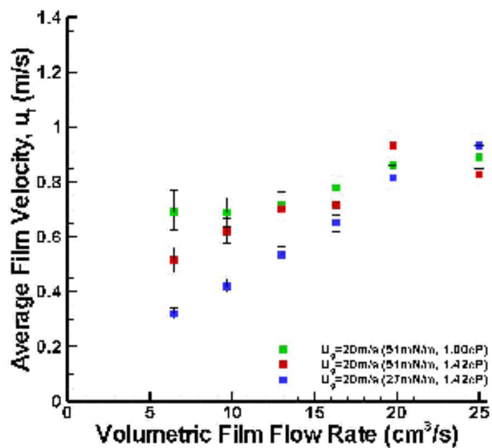
Figure 4.26. Average film velocity of all three fluids for U_g = 20 m/s.
