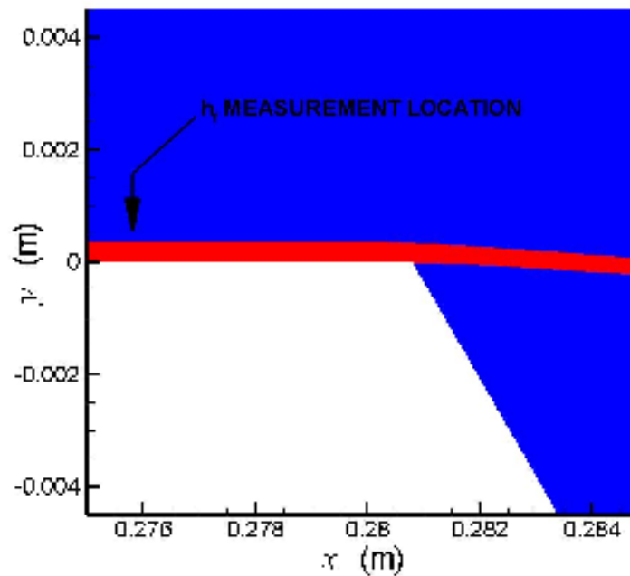
Figure 4.30. The computational results of the Volume of Fluids model for U_g = 30 m/s and \frac{\dot{V}_f}{w_f} = 2.59 cm 2 /s, with surface curvature upstream from the corner.
