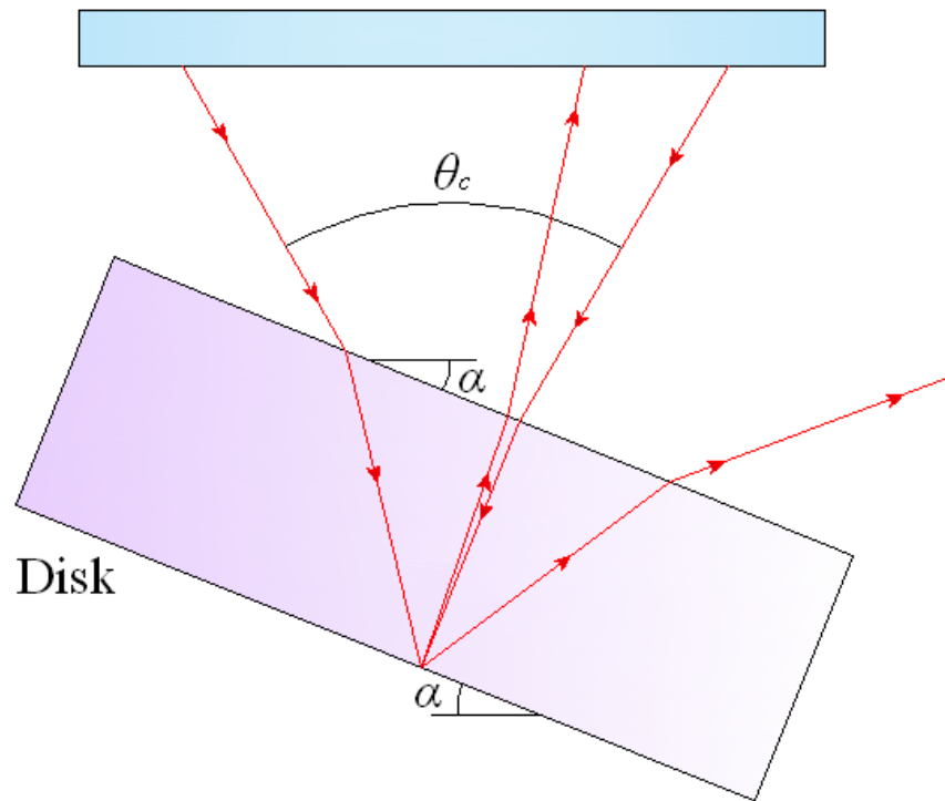
Figure 3.22. Bottom surface reflection diagram for parallel top and bottom surfaces.
