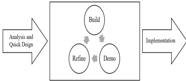
Figure 3: RAD Methodology
