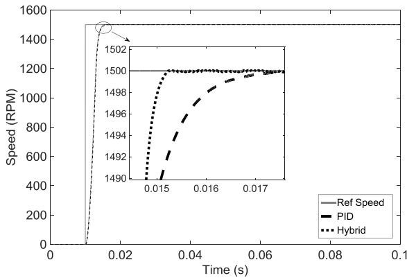
Figure 8: BLDC Motor Feedback during CW Direction for Full Load
