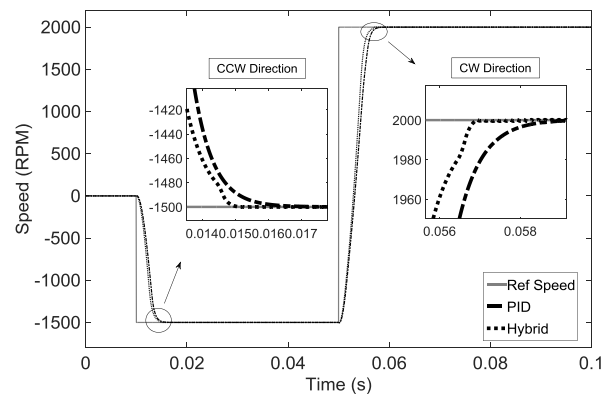
Figure 11: BLDC Motor Feedback during Full Load for both directions
