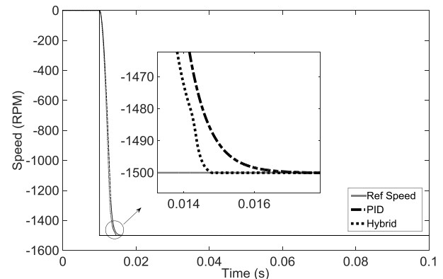
Figure 7: BLDC Motor Feedback during No Load for CCW Direction
