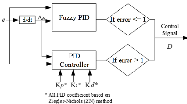
Figure 2: Proposed Controller
