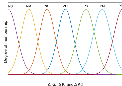
Figure 4: Membership function for \Delta K_p, \Delta K_i and \Delta K_d
