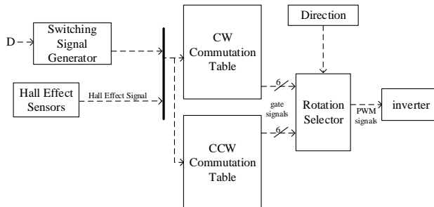
Figure 5: Direct commutation switching scheme controller
