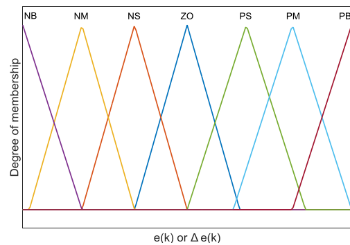
Figure 3: Membership function for e(k) and \Delta e(k)
