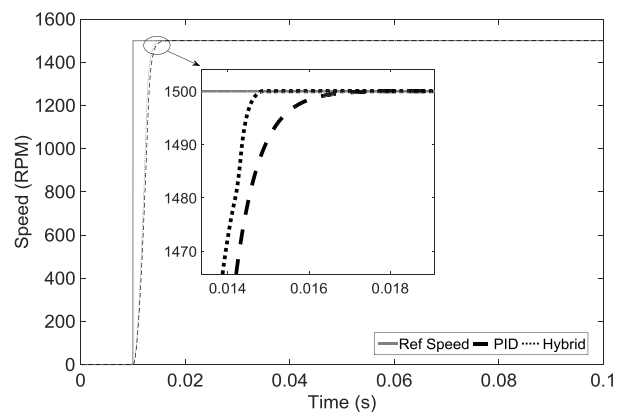
Figure 6: BLDC Motor Feedback during No Load for CW Direction
