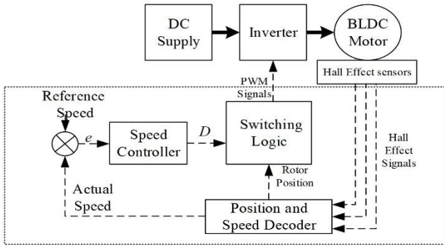
Figure 1: Speed Controller of BLDC Motor
