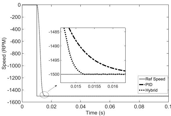
Figure 9: BLDC Motor Feedback during CCW Direction for Full Load
