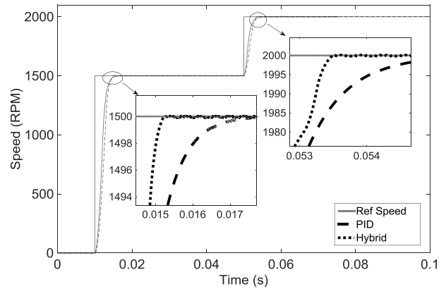
Figure 10: BLDC motor Feedback during CW Direction for Full Load
