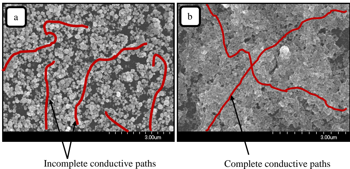
Figure 6.16 Comparison of conductive paths between microstructures. Shown are the microstructures for a) pattern I and b) pattern II. Numerous complete paths exist across (b) whereas partial paths exist across (a)
