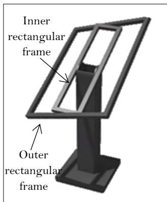
Figure 2: The 3D model of a dual axis solar tracking system
