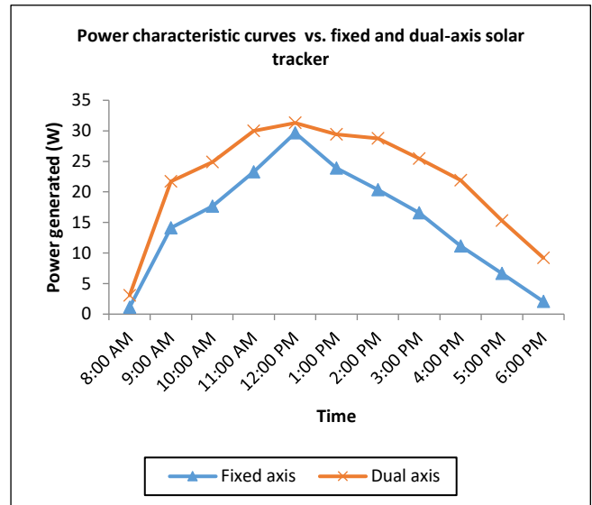
Figure 9: Solar tracking systems power generated
