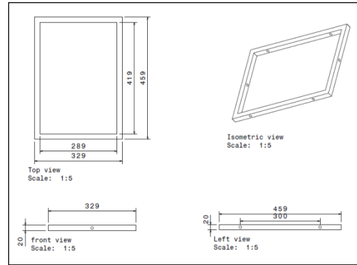
Figure 4: Outer rectangular frame
