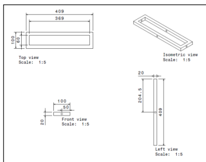
Figure 3: Inner rectangular frame
