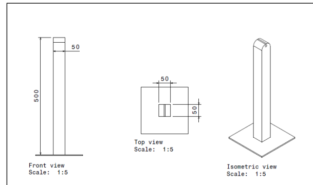
Figure 5: Solar tracker stand
