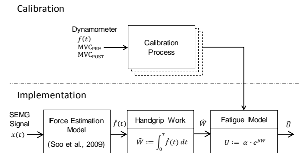
Figure 2: Overview of the proposed method for quantifying the degree of muscle fatigue using SEMG signal.
