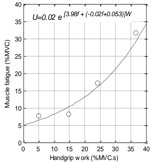
Figure 3: The fatigue model calibrated accordingly to the force loss measured with a dynamometer.
