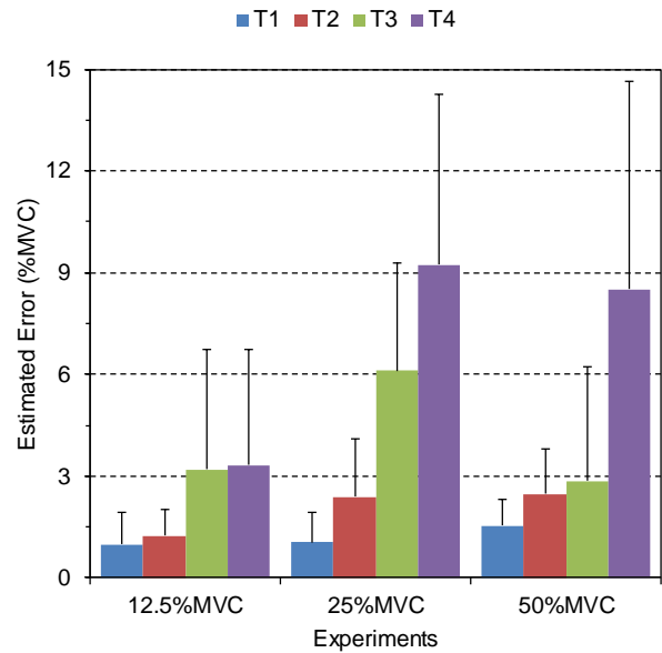
Figure 6: Error (mean and standard deviation) of the handgrip work calculated using the handgrip force measured with a dynamometer and that estimated from the SEMG signal.
