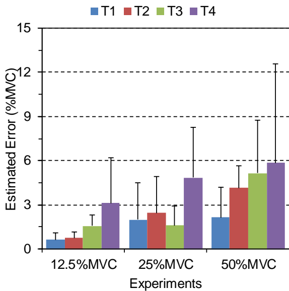
Figure 5: Mean and standard deviation for all subjects compared between the degrees of muscle fatigue estimated from the SEMG signal and the actual value measured using a dynamometer.
