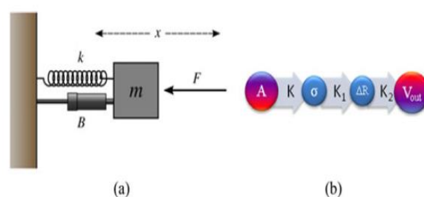
Figure 1: Piezoresistive Accelerometer Sensing Principle [3]
