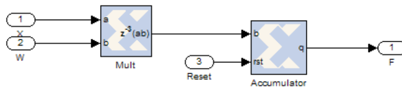
Figure 3.3. MAC hardware subsystem.
