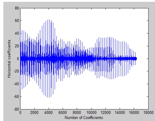
(b) Horizontal Wavelet Coefficient Before Thresholding
