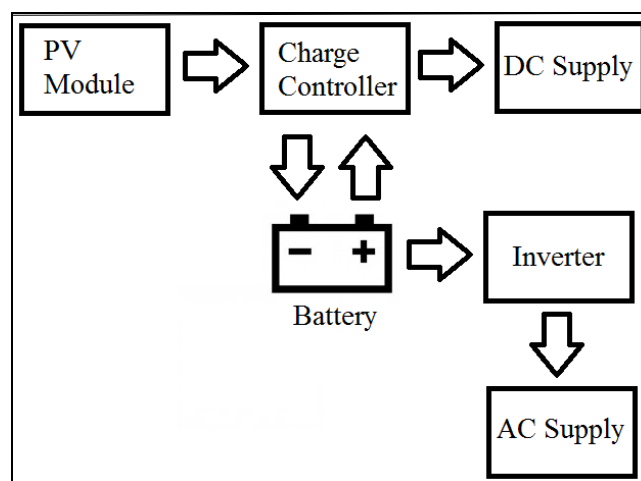
Figure 1: Block Diagram of PV System
