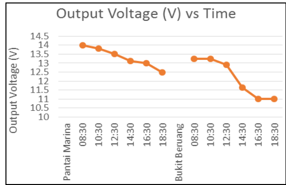
Figure 9(b): Graph output voltage vs time
