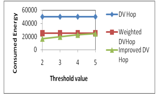
Figure 1: Comparison by varying threshold value (total anchors=50)
