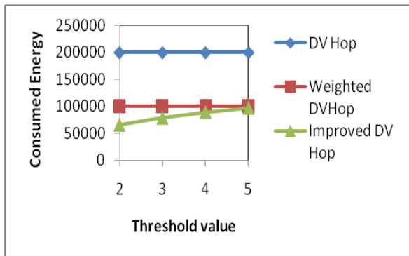
Figure 4: Comparison by varying threshold value (total anchors=200)
