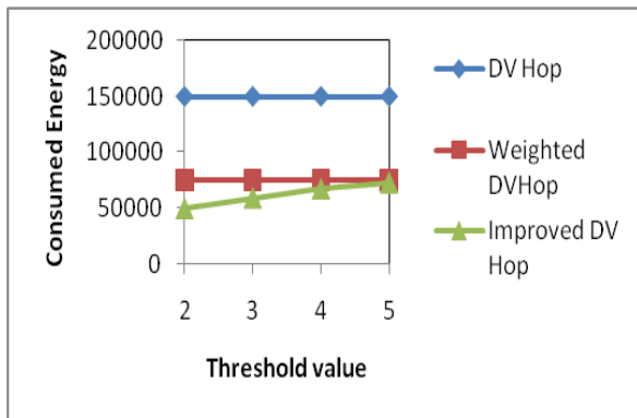
Figure 3: Comparison by varying threshold value (total anchors=150)
