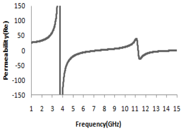
Figure 5: Real magnitude of permeability ( \mu )
