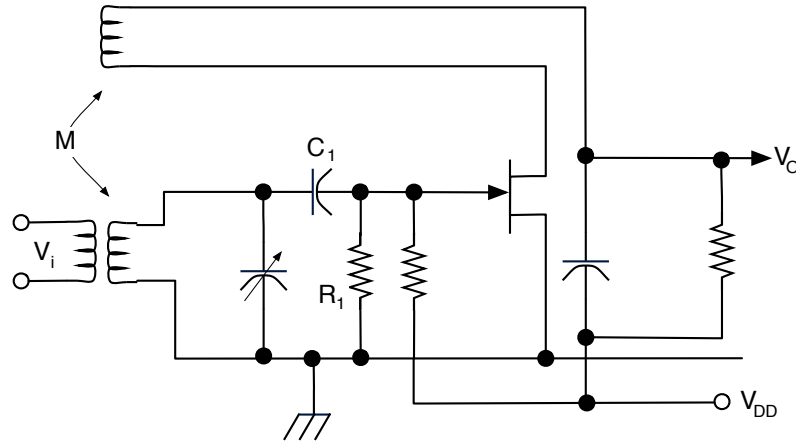
Figure 2.3 Schematic of a self-quenched super-regenerative receiver.
