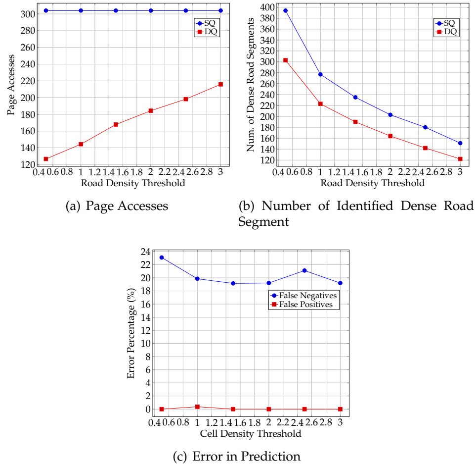
Figure 7.15 Query Performance of PDQ with Varying Road Density Threshold
