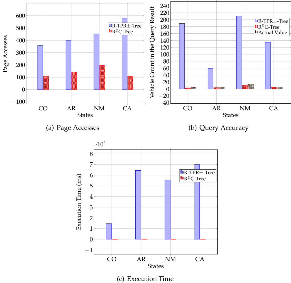
Figure 5.10 Query Performance of R^D C-tree and R\text{-TPR}\pm -tree for Different Road Topologies
