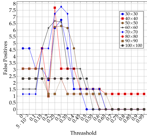
Figure 7.12 False Positives for Varying Grid Sizes, Cell Threshold and Worth County Road Network
