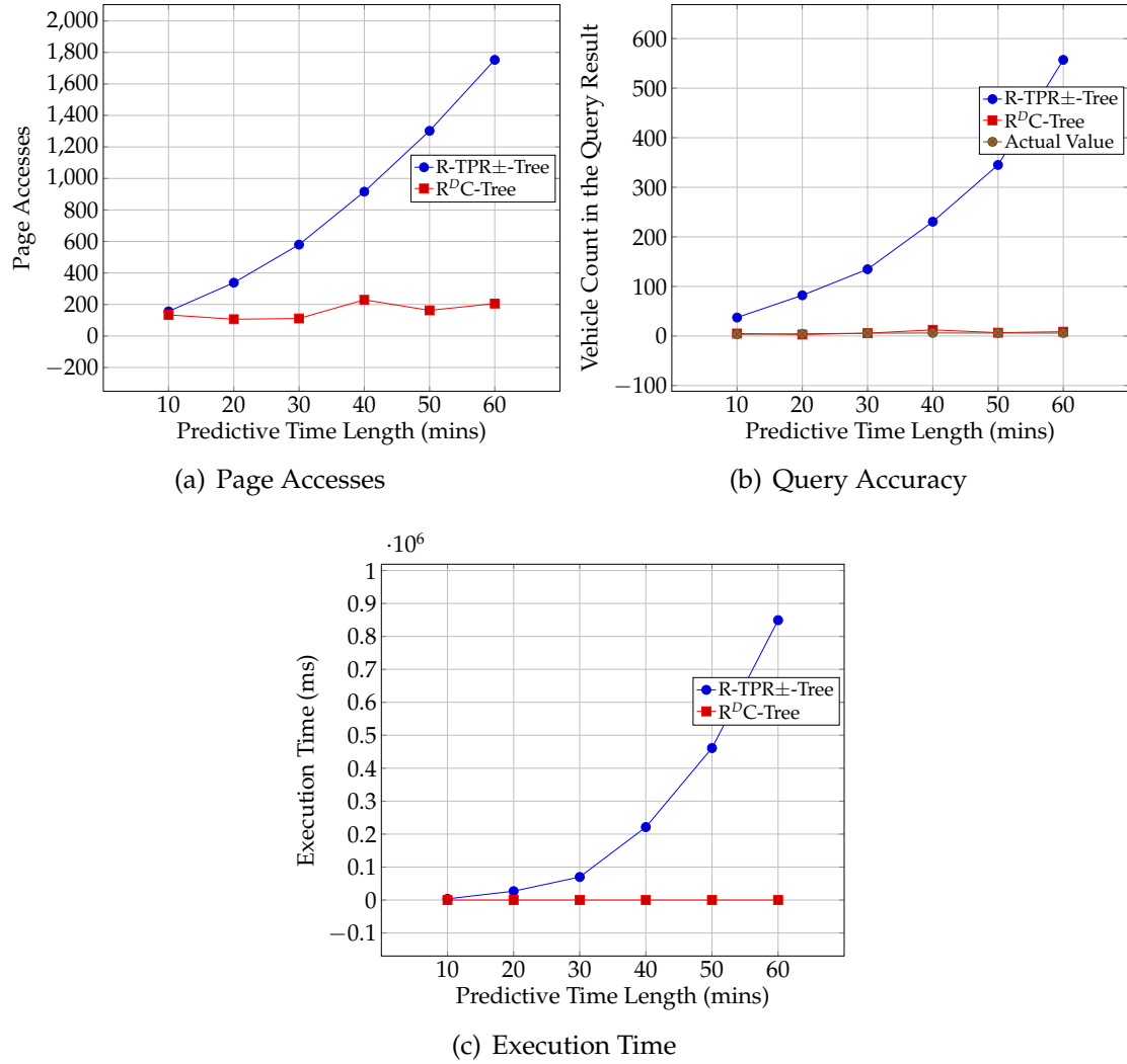
Figure 5.8 Query Performance of R D C-tree and R-TPR \pm -tree with Varying Predictive Time Length
