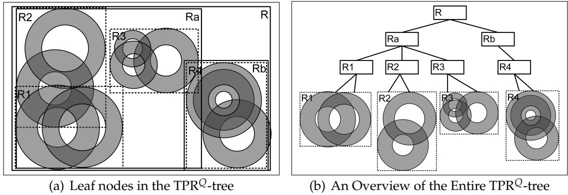
Figure 6.4 The Structure of the \text{TPR}^Q -tree
