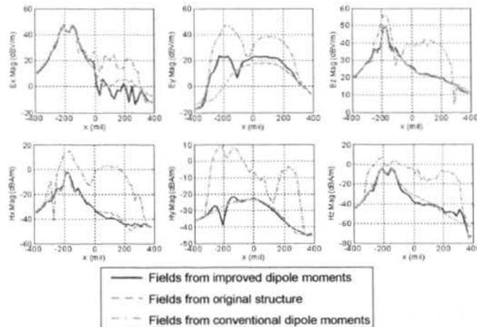
Fig. 8. Comparisons of the field magnitudes along the y=0 axis at the plane 30 mils above the ground plane from the original structure, from the improved dipole-moment sources extracted from the regularization technique, and from the dipole moments extracted from the conventional least square method.
