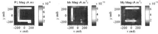
Fig. 4. Improved dipole-moment model extracted using the regularization technique.
