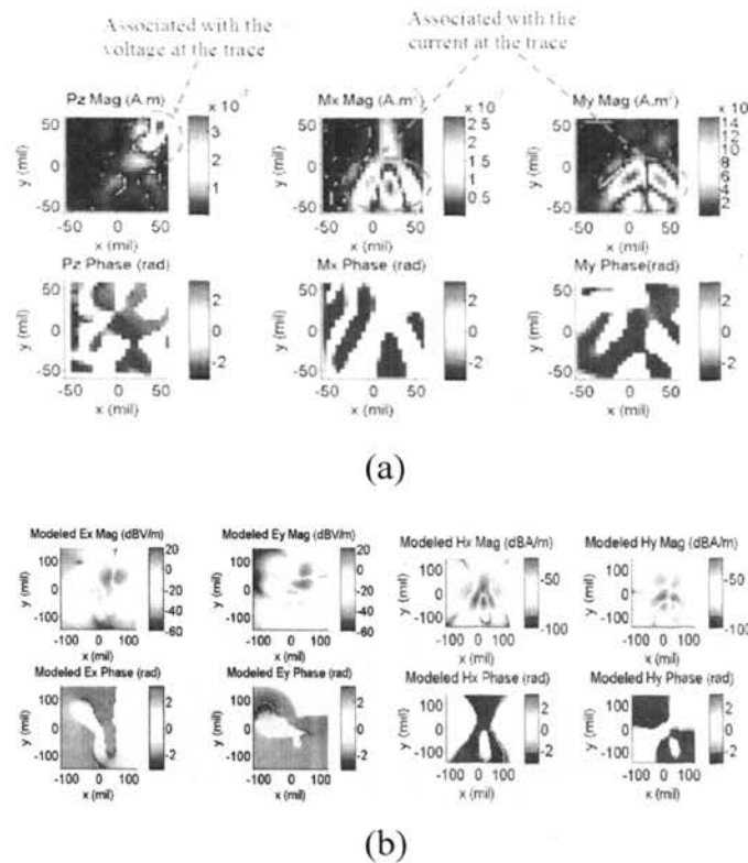
Fig. 14. Field dipoles and field generated by the dipoles. (a) Physical dipole array magnitude and phase plot, from left to right are electric dipoles Pz, magnetic dipoles Mx and magnetic dipoles My respectively. (b) The magnitude and phase of electric and magnetic field generated by physical dipoles.
