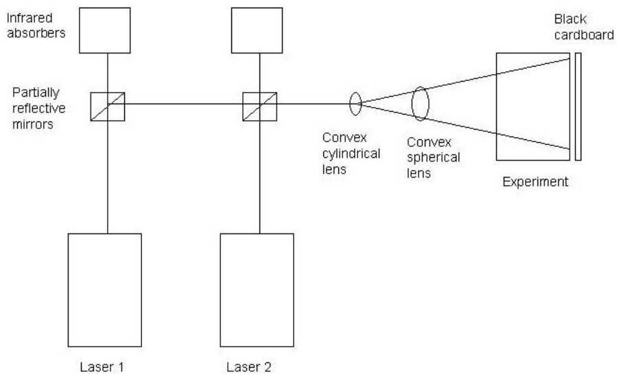
Figure 3-9: PIV optics.
