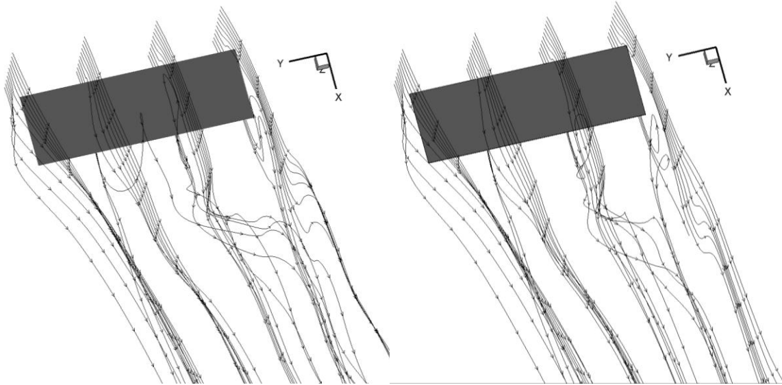
Figure 4-18: Streamlines at Re_c = 500 (left) and 5,000 (right.)
