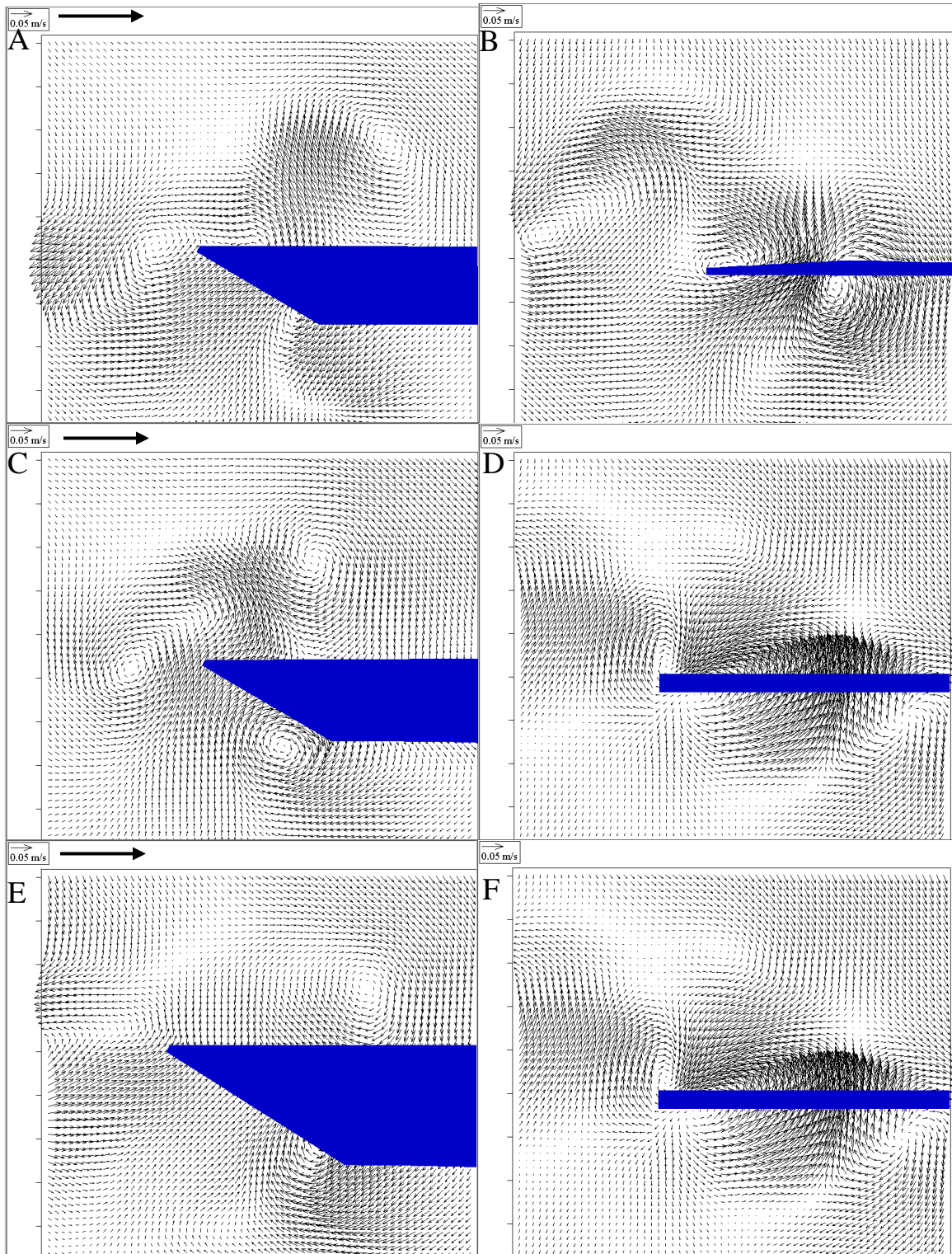
Figure 4-32: Effect of wing shape. Left and right columns are at one quarter and one half period, respectively. The three rows are 50mm chord rectangle, 75mm chord semi-ellipse, and 75mm chord rectangle.
