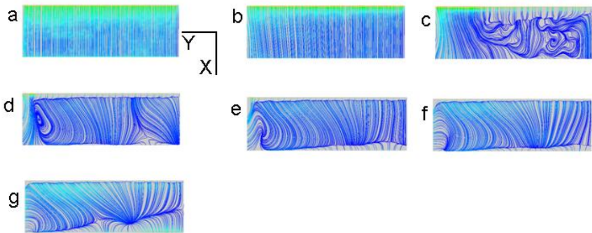
Figure 4-19: Suction surface streamtraces for non-cambered rectangular wing. Flow is from top to bottom, tip is left and root is right. Beginning at top left, \alpha = 0^\circ, 10^\circ, 20^\circ, 30^\circ, 35^\circ, 40^\circ, and 45^\circ . Colors indicate shear stress.
