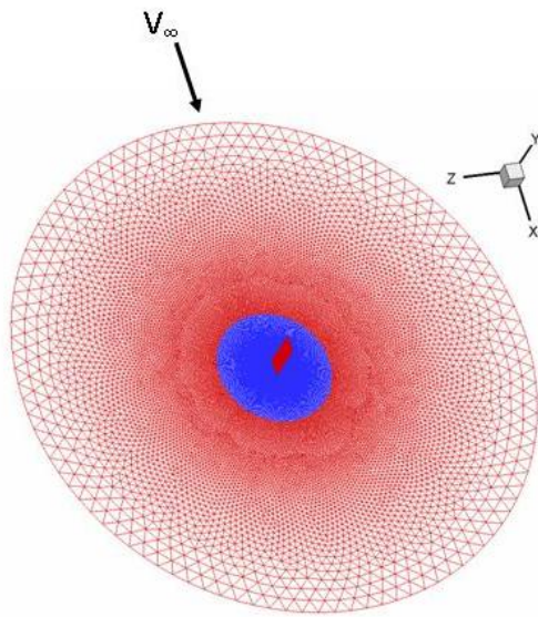
Figure 4-1: Cross section of computational domain, showing the wing and circular base surfaces.
