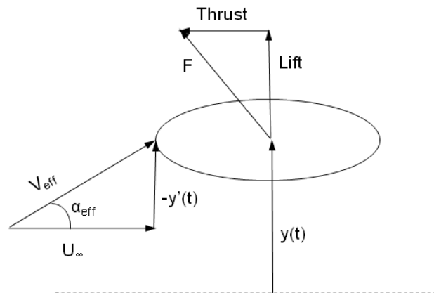
Figure 2-4: Knoller-Betz effect.
