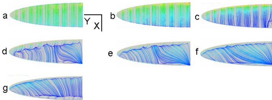
Figure 4-22: Suction surface streamtraces for cambered semi-ellipse wing. Flow is from top to bottom, tip is left and root is right. Beginning at top left, \alpha = 0^\circ, 10^\circ, 20^\circ, 30^\circ, 35^\circ, 40^\circ, and 45^\circ . Colors indicate shear stress.
