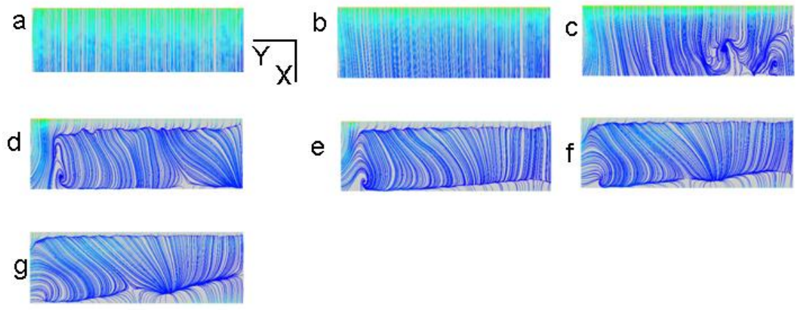
Figure 4-20: Suction surface streamtraces for cambered rectangular wing. Flow is from top to bottom, tip is left and root is right. Beginning at top left, \alpha = 0^\circ, 10^\circ, 20^\circ, 30^\circ, 35^\circ, 40^\circ, and 45^\circ . Colors indicate shear stress.
