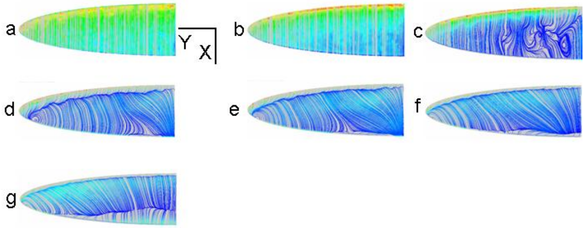
Figure 4-21: Suction surface streamtraces for non-cambered semi-ellipse wing. Flow is from top to bottom, tip is left and root is right. Beginning at top left, \alpha = 0^\circ, 10^\circ, 20^\circ, 30^\circ, 35^\circ, 40^\circ, and 45^\circ . Colors indicate shear stress.
