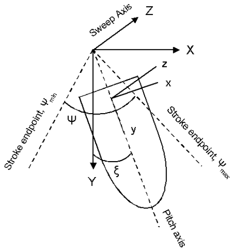
Figure 3-7: Coordinate system.
