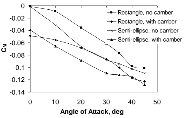
Figure 4-10: Moment coefficient about quarter-chord.
