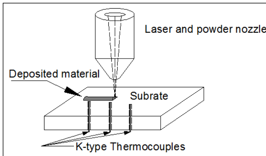
Figure 3.1. Scheme for locating thermocouples on the substrate
