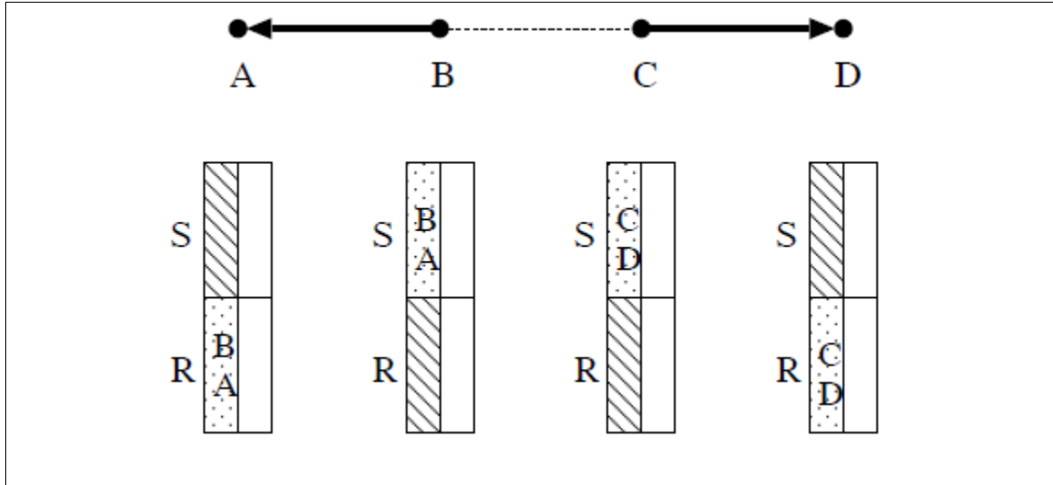
Fig.2.13 The SlotAssignment algorithm would allow C \rightarrow D and B \rightarrow A to occur at the same time.
