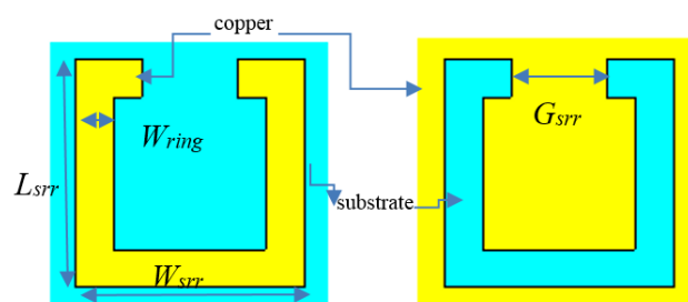
Figure 1: The design of the SRR, (a) basic SRR, (b) complimentary SRR
