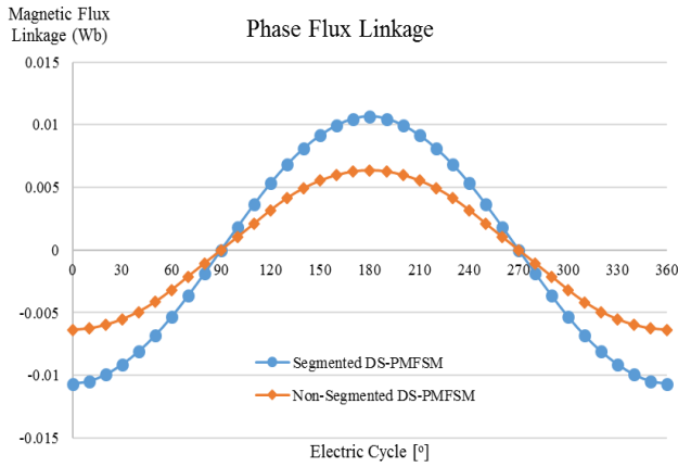
Figure 5: Phase flux linkage comparison
