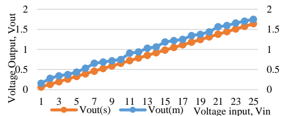
Figure 10: Vout test & Vout simulation vs. Vin
