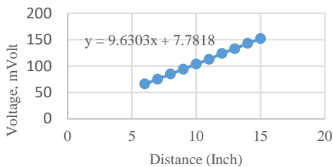
Figure 11: Voltage ultrasonic vs distance
