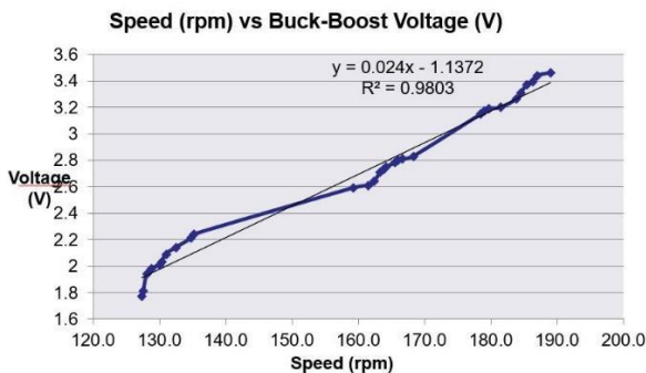
Figure 7 Speed(rpm) Vs Generated Voltage(V) for Light Weight, Medium Weight, and Heavy Weight Riders.
