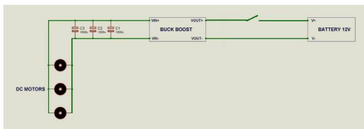
Figure 2: ReGen Schematic Diagram
