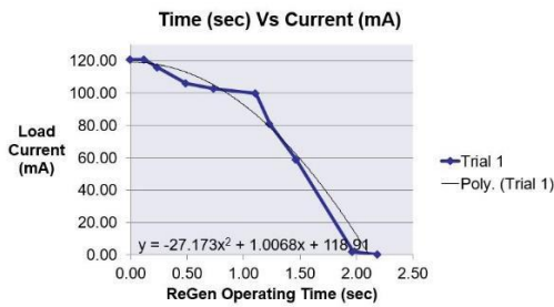
Figure 6: Buck-Boost Current(mA) Vs Battery Charging Time(Sec) for Heavy Weight Rider
