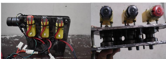
Figure 3: Trolley Assembly
