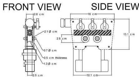
Figure 1: Trolley Design
