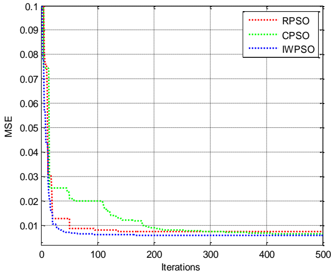
Figure 6: Convergence Curve of the Training Algorithms
