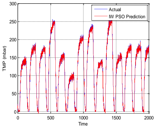
Figure 9: TMP model testing result
