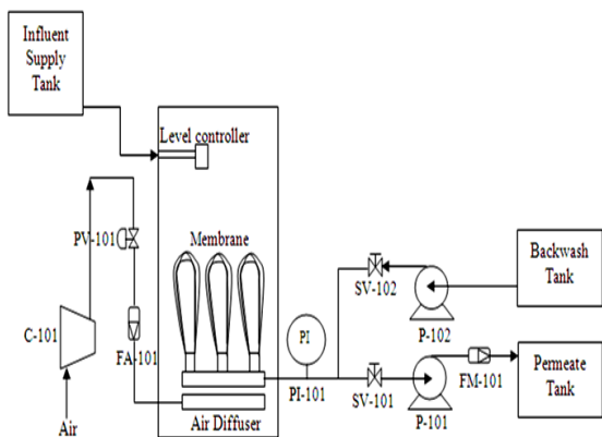
Figure 1: Plant Schematic
