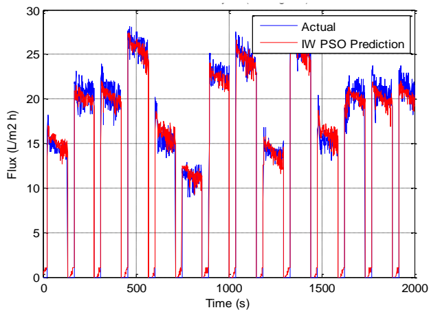
Figure 10: Permeate flux testing result
