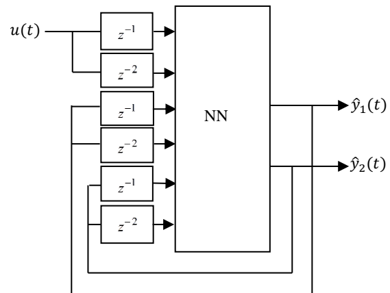
Figure 3: Recurrent Structure
