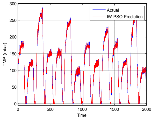
Figure 7: TMP model training result
