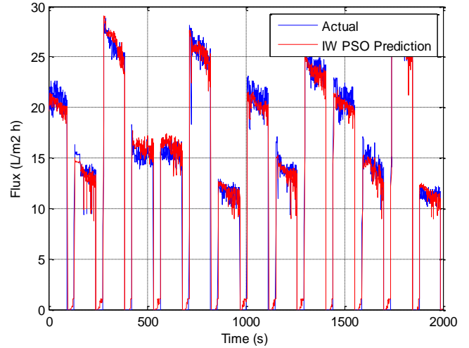
Figure 8: Permeate flux training result
