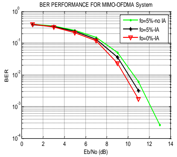
Figure 3: BER performances for STFBC MIMO-OFDMA system with and without IA scheme using different FO
