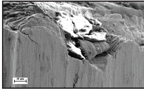
Fig. 4 Chipping of ceramic cutting tools when cutting at VC = 200 m/min, f = 0.06 mm/rev and depth of cut = 0.4 mm
