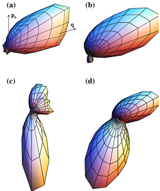
FIG. 1 (color online). Three-dimensional angular distribution of electrons ejected in 1 MeV/amu \text{Li}^{3+} + \text{He} collisions. (a) Calculation for electrons ejected in single ionization; (b) calculation for electrons ejected in independent transfer ionization; (c) experimental data for electrons ejected in transfer-ionization; (d) calculation for electrons ejected in the independent and ee transfer-ionization processes.
