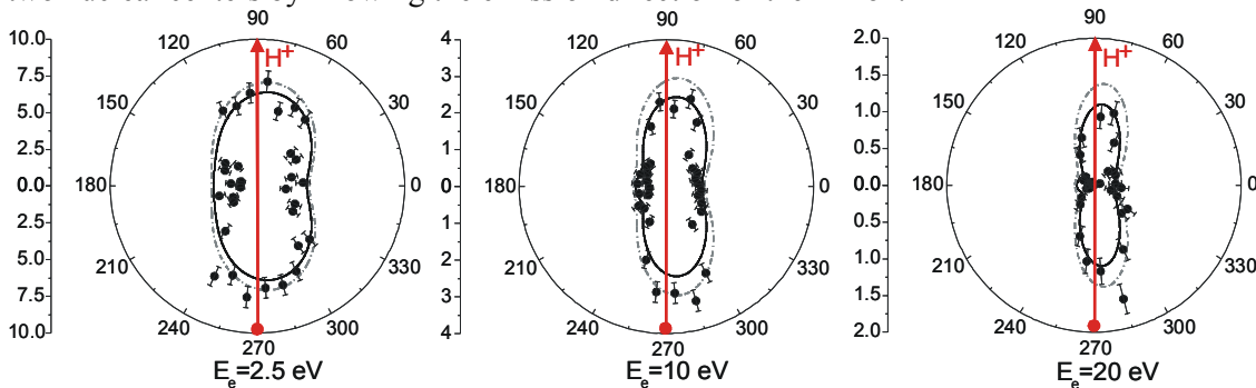
Figure 6. Electron angular distributions for H_2 molecules oriented perpendicular to the incoming projectile beam and for E_e = 2.5 eV, 10 eV and 20 eV. The arrows indicate the emission direction of the detected H^+ fragment. CDW-EIS calculation: “molecular” (solid lines), “effective” atomic (dashed lines). The theoretical FDCS have been integrated over \mathbf{q}_\perp . The cross sections are given in 10^{-20} \text{ cm}^2/\text{eV} . The data have been normalised to the “molecular” CDW-EIS cross section around 90^\circ .
