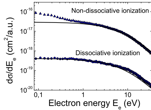
Figure 2. Electron energy distributions for single ionization of \text{H}_2 by 6 MeV proton impact. Triangles: non-dissociative ionization. Circles: dissociative ionization. Solid lines: CDW-EIS results.
