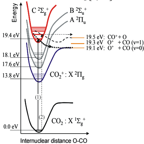
Figure 4. Schematic potential curves for CO_2 and CO_2^+ with the lowest dissociation limits of CO_2^+ . The suggested mechanism for CO_2 \rightarrow O^+ + CO + e^- by predissociation (curve crossing) of the C^2\Sigma_g^+ state of CO_2^+ is illustrated by (1). For CO_2 \rightarrow CO^+ + O + e^- the analogous mechanism is shown by (2).
