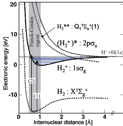
Figure 1. Schematic potential curves for \text{H}_2 and \text{H}_2^+ illustrating the single ionization pathways.
