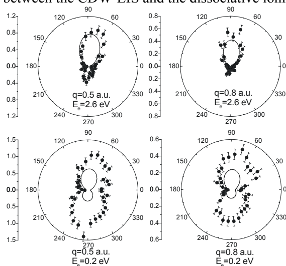
Figure 3. FDCS for electrons emitted into the scattering plane for non-dissociative ionization of H_2 by 6 MeV proton impact. Upper row: The electron energy E_e = 2.6 eV is fixed and the values of the momentum transfer are q = 0.5, 0.8 a.u.. Lower row: E_e = 0.2 eV, same values of q . Solid lines: CDW-EIS results. The cross sections are given in 10^{-18} \text{ cm}^2/\text{au}^2 .
