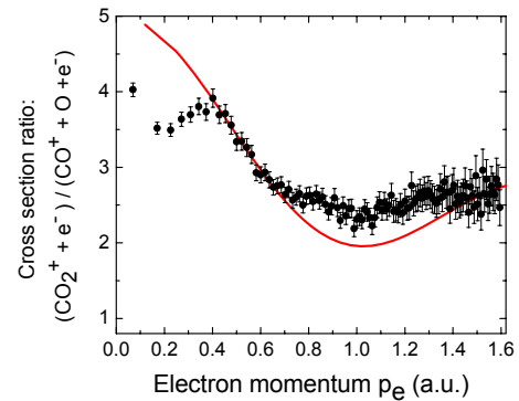
Figure 5. Ratio of the electron momentum distribution for non-dissociative single ionization of CO_2 to the one for fragmentation into CO^+ + O . Solid line: calculation of the simple interference term [1 + \sin(p_e R)/(p_e R)] with R = 4.38 \text{ \AA} , scaled on the data at p_e = 0.4 \text{ a.u.}
