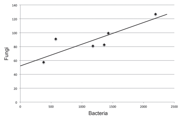
Fig. 2. Plot of the concentration of fungal PLFA (18:2 \omega 6,9) compared to bacterial PLFAs, yielding a correlation of r = 0.85 ( r^2 = 0.72 ).
