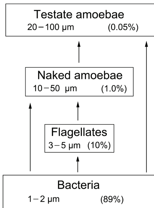
Fig. 1. Diagram of a tundra, bacterial-based protozoan trophic hierarchy showing the typical size range of each group of biota ( \mu\text{m} ), percent of total C-biomass in parentheses, and predator prey relationships (arrows) based on data in this paper. As in trophic webs of higher organisms, biota at increasingly higher levels of the hierarchy are larger, but account for increasingly less of the total C-biomass in the community of organisms. Bacterial-based protozoan trophic hierarchies are often more complex, because higher-order predators also prey on bacteria at the base of the food chain in some cases, in addition to preying on intermediate taxa in the hierarchy.
