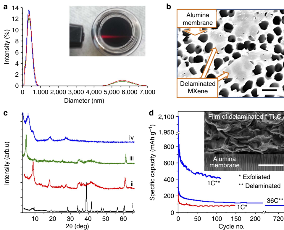
Figure 4 | Delaminated f\text{-Ti}_3\text{C}_2 and its properties. (a) Particle size distribution in aqueous colloidal solution; inset shows Tyndall scattering effect in the solution. (b) SEM images of f\text{-Ti}_3\text{C}_2 flakes on an alumina membrane. (c) XRD patterns of (i) \text{Ti}_3\text{AlC}_2 , (ii) exfoliated, (iii) DMSO intercalated and (iv) delaminated \text{Ti}_3\text{C}_2 . Note the disappearance of the non-basal peaks at \sim 60^\circ in iv. (d) Comparison of the performance of exfoliated and delaminated f\text{-Ti}_3\text{C}_2 as anode material in Li-ion batteries. Inset shows SEM image of an additive-free film of delaminated f\text{-Ti}_3\text{C}_2 filtered through the membrane. Scale bars, 0.4\ \mu\text{m} in b ; 4\ \mu\text{m} in inset d .
