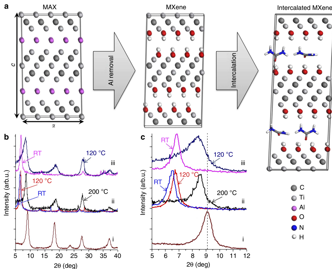
Figure 1 | Evidence of MXene intercalation. (a) Schematic of synthesis and intercalation of f\text{-Ti}_3\text{C}_2 . First, the Al layer is removed from the corresponding MAX phase in 50% aqueous HF. The f\text{-MXene} is then treated with an intercalant (urea is shown as an example) yielding intercalation compounds. (b) XRD patterns of f\text{-Ti}_3\text{C}_2 : (i) as received, before any treatment, (ii) after HM in DMF treatment, washed with DMF, (iii) after HM treatment, washed with ethanol and dried in different conditions. (c) Zoom-ins of b in the 5\text{--}12^\circ 2\theta range showing (0002) peaks.
