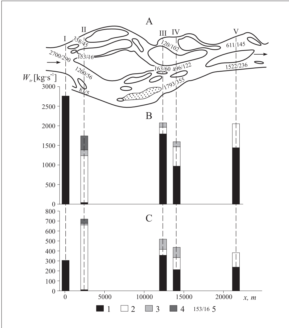
Fig. 3. Sediment transport capacity changes (with respect to suspended sediment) W_{tr} along the Yakutskoe bifurcation on the Lena River (Alexeevskiy, Chalov 2004)
