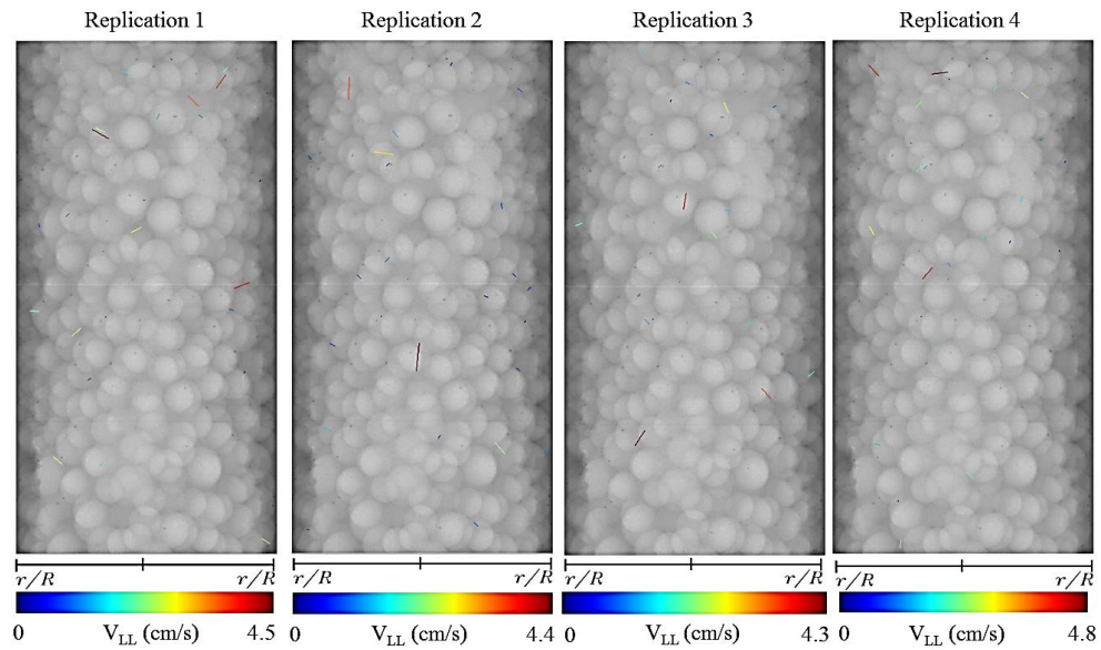
Figure 5.3. The identified 2D particle paths, V_{LL} in every replication, and color bars for V_{SL} = 1.11 \pm 2\% cm/s
