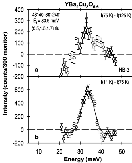
FIG. 9. Constant- q scans at (0.5, 1.5, 1.7) rlu above and below T_c for \text{YBa}_2\text{Cu}_3\text{O}_{6.6} with the crystal in the [h, 3h, l] zone. (a) The temperature difference between 75 K ( T_c + 12 K) and 125 K. (b) The temperature difference between 11 K ( T_c - 52 K) and 75 K. The solid line is a Gaussian fit to the data.
