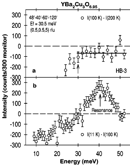
FIG. 21. Difference spectra in constant- q scans at (0.5, 0.5, 5) rlu above and below T_c for \text{YBa}_2\text{Cu}_3\text{O}_{6.95} . (a) The difference spectrum between 100 K ( T_c + 8 K) and 200 K. Note that there are no observable features above the background around 40 meV in the normal state, again confirming no precursor of the resonance. (b) The temperature difference between 11 K ( T_c - 81 K) and 100 K.
