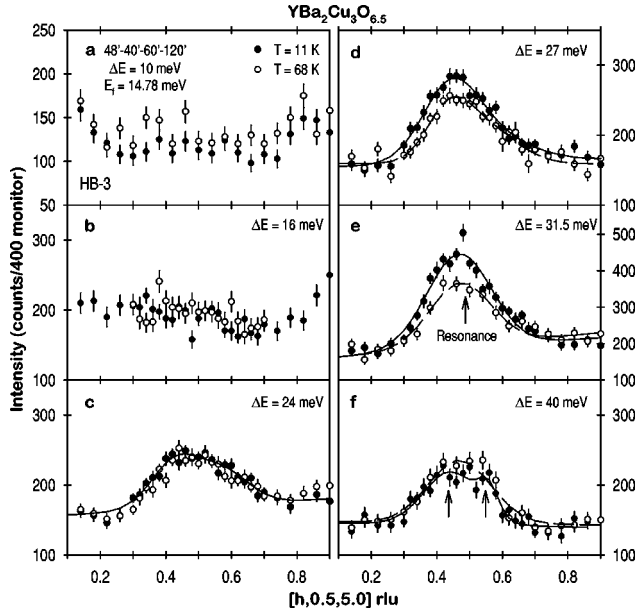
FIG. 8. Constant-energy scans along the [h,0.5,5.0] direction for \text{YBa}_2\text{Cu}_3\text{O}_{6.5} . The energy transfers are \hbar\omega = 10 meV (a), 16 meV (b), 24 meV (c), 27 meV (d), 31.5 meV (e), and 40 meV (f). The flattish top profiles indicative of the incommensurate spin fluctuations are observed at \hbar\omega = 24 meV both above and below T_c . In the superconducting state, flattish top profiles are also observed above the resonance \hbar\omega = 40 meV. The solid lines are Gaussian fits to the data, and the arrows in (c) and (f) mark the fitted incommensurate positions.
