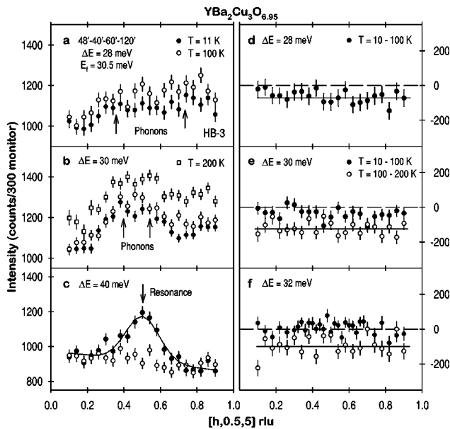
FIG. 22. Constant-energy scans along the [h, 0.5, 5] direction at various temperatures for \text{YBa}_2\text{Cu}_3\text{O}_{6.95} . The energy transfers are \hbar\omega = 28 meV (a), 30 meV (b), and 40 meV (c). The weak structures in (a) and (b) at 11 K marked by arrows are nonmagnetic scattering. (d) The temperature difference spectrum for \hbar\omega = 28 meV between 10 K and 100 K shows no observable feature around (\pi, \pi) . (e) and (f) suggest no discernible magnetic scattering above and below T_c at \hbar\omega = 30 and 32 meV. In addition, no evidence for incommensurate spin fluctuations is found below \hbar\omega = 32 meV. The solid lines are Gaussian fits to the data and guides to the eye.
