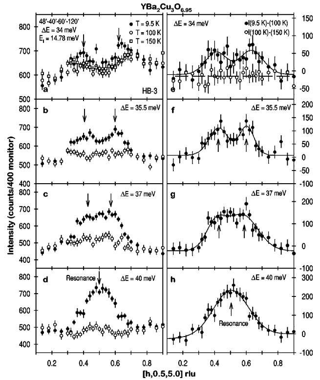
FIG. 23. High-resolution constant-energy scans along the [h, 0.5, 5] direction at various temperatures for \text{YBa}_2\text{Cu}_3\text{O}_{6.95} . The energy transfers are \hbar\omega = 34 meV (a), 35.5 meV (b), 37 meV (c), and 40 meV (d). The enhancement of the scattering from 100 K to 9.5 K is marked by arrows. (e) The filled circles show the difference between 9.5 K ( T_c - 82.5 K) and 100 K. The open circles are the difference between 100 K and 150 K. Therefore, while there is no discernible magnetic intensity in the normal state, clear incommensurate spin fluctuations are observed in the superconducting state. (f) and (g) show the presence of incommensurate magnetic scattering at \hbar\omega = 35.5 and 37 meV with the incommensurability marked by arrows. (h) shows the commensurate resonance. The solid and dashed lines are Gaussian fits to the data and guides to the eye, respectively.
