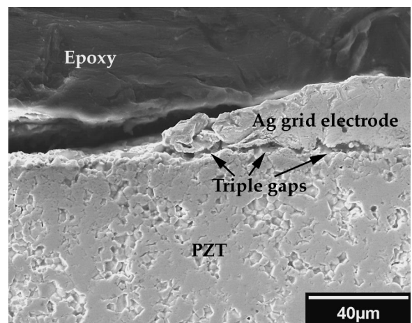
FIG. 4. SEM micrograph of the polished sample cross section showing the triple gaps between the ceramic and the grid electrode (from Ref. 8).
