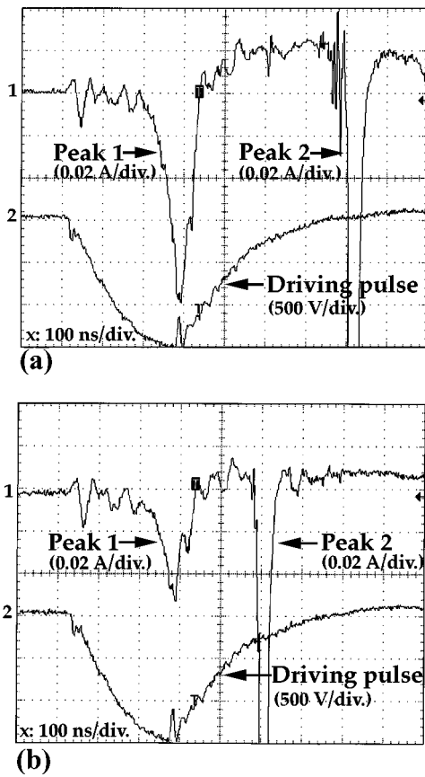
FIG. 1. Typical emission current traces when a negative driving pulse is applied to the sample with no extraction potential on the collector. Note that (a) and (b) are two consecutive recordings (from Ref. 8).
