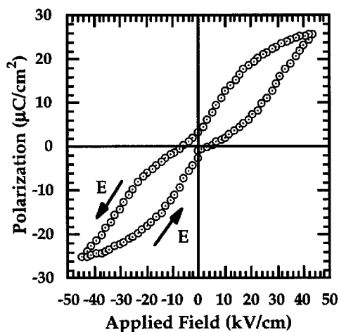
FIG. 7. Hysteresis loop of PZT EC-64 with grid electrodes measured at room temperature (from Ref. 8).
