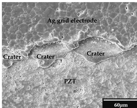
FIG. 2. SEM micrograph of the emission surface after the emission studies (plasma emission region).
