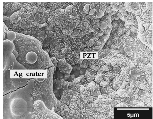
FIG. 3. Higher magnification SEM micrograph of the small particles accumulated near the crater on the grid electrode (plasma emission region).
