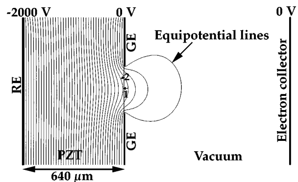
FIG. 6. The potential distribution inside and outside the ferroelectric. [RE: rear electrode, GE: grid electrode ( 300 \mu\text{m} ).]
