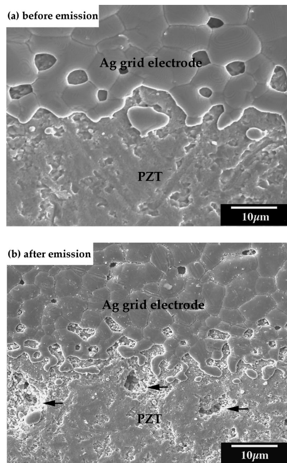
FIG. 5. SEM micrographs of the emission surface (a) before and (b) after the emission studies (ferroelectric emission region).
