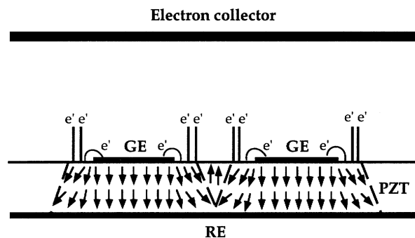
FIG. 8. Schematic diagram of the domain switching distribution after a driving pulse is applied to the ferroelectric sample. (RE: rear electrode, GE: grid electrode.)
