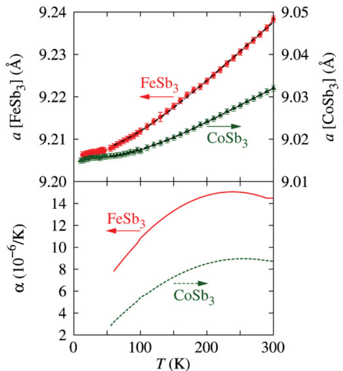
FIG. 6. (Color online) Top: The temperature dependence of the lattice parameter a for FeSb 3 (red) and CoSb 3 (green), and the corresponding polynomial fit (black). Bottom: The thermal expansion coefficient \alpha of FeSb 3 and CoSb 3 .
