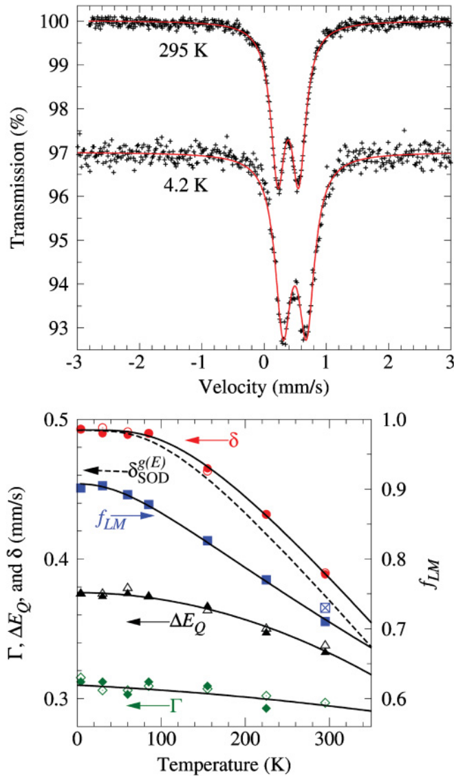
FIG. 7. (Color online) Top: The Mössbauer spectra of FeSb 3 obtained on a 1.5 \mu\text{m} film. Bottom: The fit parameters obtained from the spectra of the \sim 1 and \sim 1.5 \mu\text{m} films (open and closed symbols), respectively. The errors are the size of the symbols. The crossed square indicates the f_{LM} obtained directly from the ^{57}\text{Fe} NIS at 295 K. The dashed line indicates the second-order Doppler shift obtained from the DPS; see text. The lines for the Doppler shift and f_{LM} are Debye model fits. 41 The lines for \Delta E_Q and \Gamma are quadratic polynomial fits given as a guide for the eye.
