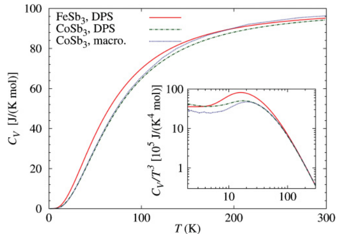
FIG. 10. (Color online) A comparison of the total heat capacity, calculated from the DPS of \text{FeSb}_3 (red solid lines) and from the DPS and theoretical calculations for \text{CoSb}_3 (green dash-dotted lines), and the macroscopic measured heat capacity of \text{CoSb}_3 (blue dotted lines).
