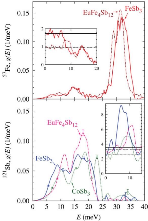
FIG. 9. (Color online) Comparison of the DPS measured with the ^{57}\text{Fe} resonance at 295 K for \text{FeSb}_3 and \text{EuFe}_4\text{Sb}_{12} (top) and with the ^{121}\text{Sb} resonance at 25 K for \text{FeSb}_3 , \text{CoSb}_3 , and \text{EuFe}_4\text{Sb}_{12} (bottom). The insets show the reduced partial DPS g(E)/E^2 in units of 10^{-4}/\text{meV}^3 , and the low-energy fit between 0 and 4 meV for the Debye levels, indicated by the same type of lines. The differences in the Debye levels for Fe and Sb in \text{FeSb}_3 and \text{EuFe}_4\text{Sb}_{12} are due to the different masses of the elements; see Eq. (1).
