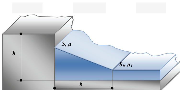
Fig. 1. Drifted snow load zone in the places of height discontinuity (according to codes of structural design)
