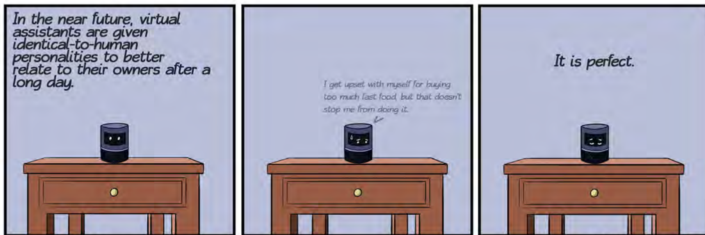
Artificial Intelligence
