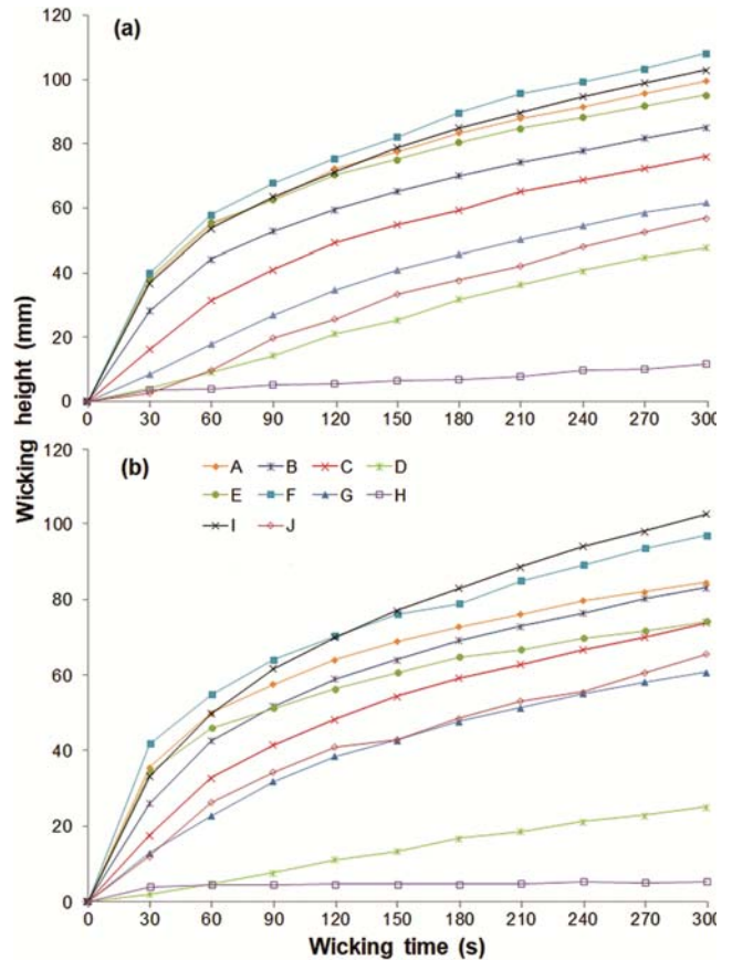
Fig. 3 — Wicking height and time curve in 300 s (a) wale, and (b) course
