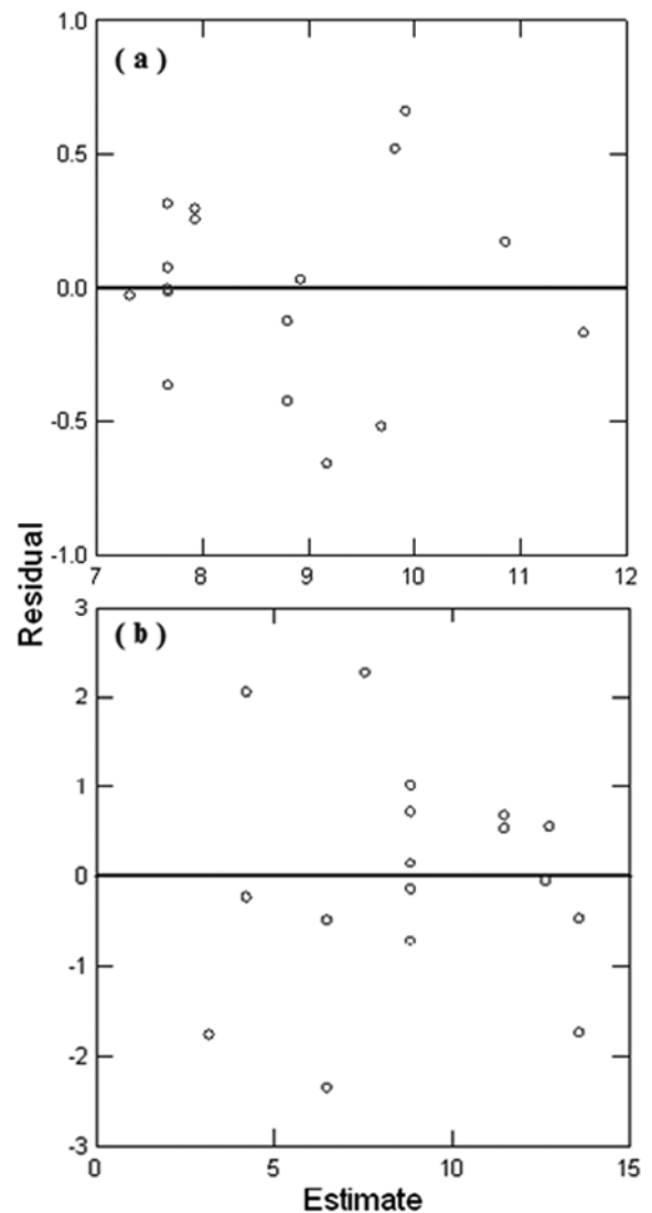
Fig. 3 — Plot of residuals vs. predicted value for (a) mass loss (%) of fabric after abrasion and (b) loss in fabric appearance after abrasion
