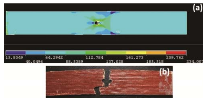
Fig. 1 — Comparison of stress distribution between finite element model (a), and experimental sample (b), for axial laminates 4 mm hole sample
