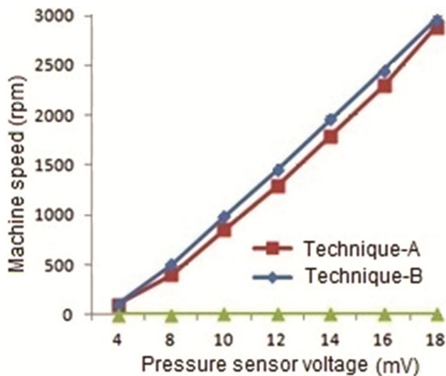
Fig. 3 — Pressure sensor voltage and machine speed comparison graph
