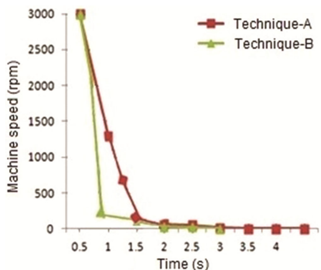
Fig. 5 — Machine speed and time comparison graph at braking
