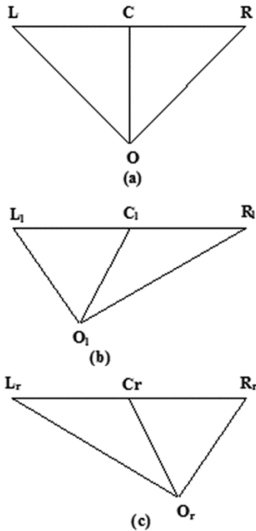
Fig. 2 — Spinning triangle of (a) normal path yarn, (b) left diagonal path yarn and (c) right diagonal path yarn
