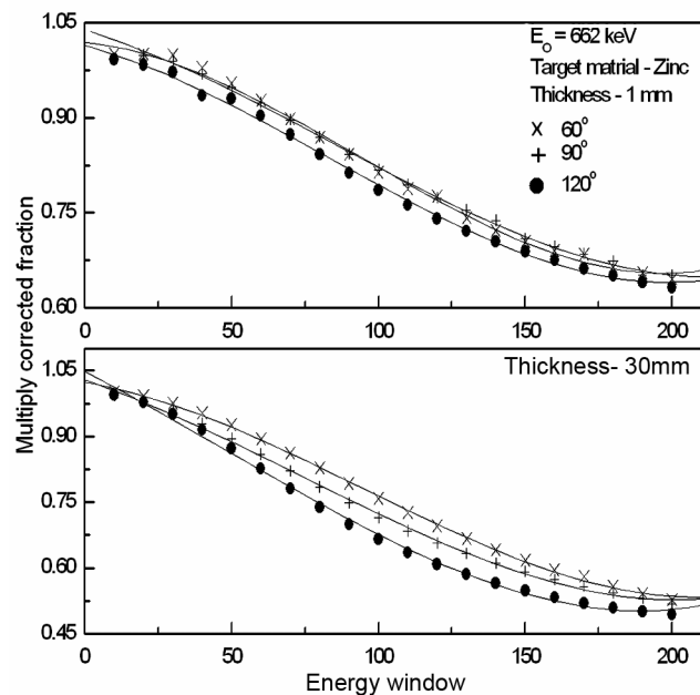
Fig. 7 — Plot of multiply scattered fractions (MSF) as function of energy window around the Compton scattered peak centroid for 662 keV photon energy at scattering angles of 60°, 90° and 120° for target thickness of 1 mm and 30 mm
