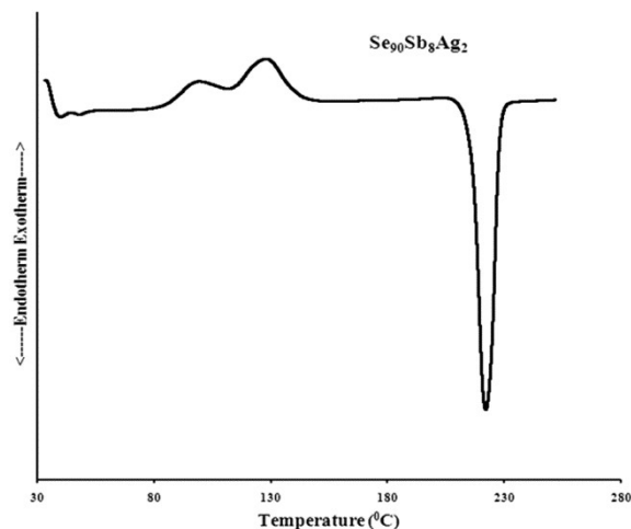
Fig. 1 — DSC thermogram for glassy \text{Se}_{90}\text{Sb}_8\text{Ag}_2 alloy for heating rate (15 °C/min).
