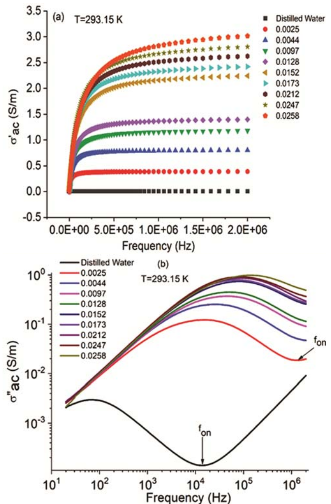
Fig. 2 – Plots of (a) real part \sigma'_{ac} and (b) imaginary part \sigma''_{ac} of complex ac conductivity against frequency for different weight fractions of [BMiM][Cl] in distilled water at 293.15 K.
