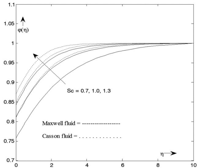
Fig. 10 — Effect of variation of the Schmidt number on concentration profile when K = 0.1, M = 1, k_1 = 0.2, k_2 = 0.1 .
