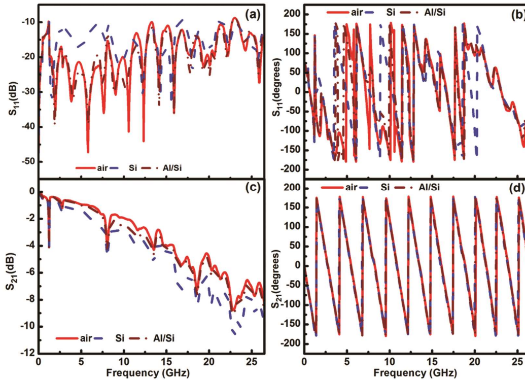
Fig. 4 – S-parameters for microstrip line with no loading (air), Si loading, Al/Si loading, (a) S_{11} (dB), (b) S_{11} (degrees), (c) S_{21} (dB) and (d) S_{21} (degrees).
