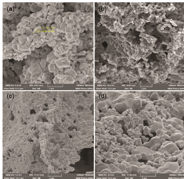
Fig. 2 – SEM image of CuO nanoparticles; (a) 450 °C, (b) 550 °C, (c) 650 °C and (d) 800 °C.
